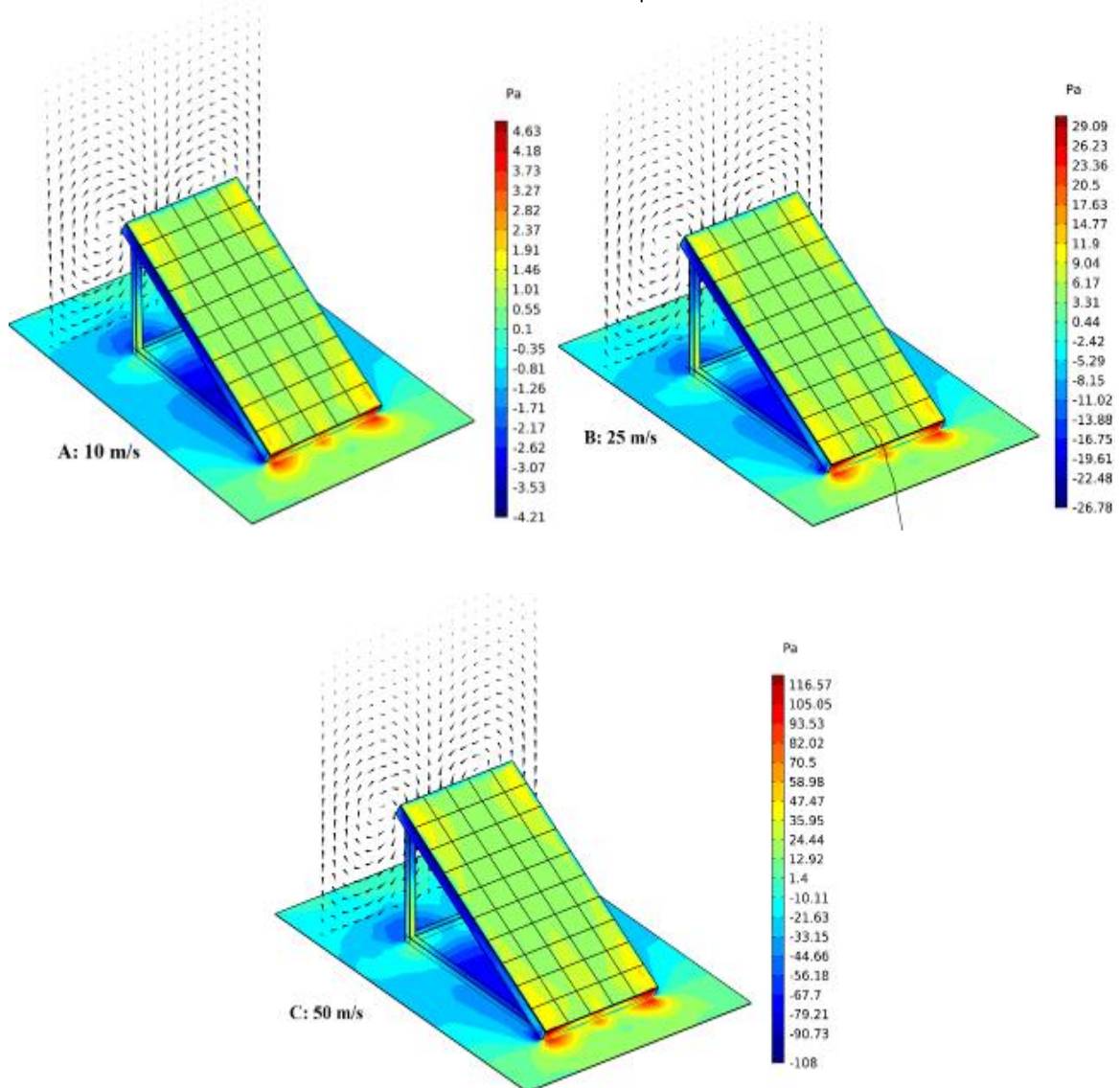
Figure 4. The contours of surface pressure and the speed components of the plane are 6 cm behind the panel
