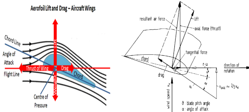
Figure (4). Aerfoil lift action.
