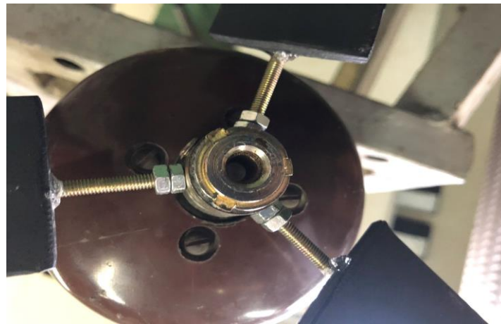
Figure (7). Blades pitch adjustment.
