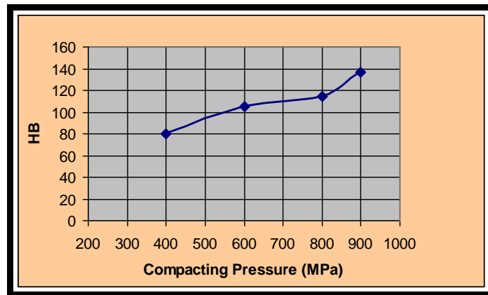
Figure (9): Effect of compacting pressure on the HB values of the sintered alloy sample.
