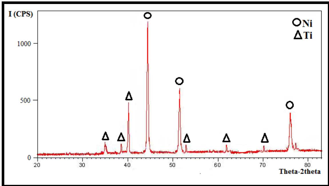
Figure (5): XRD pattern of the green compact sample.
