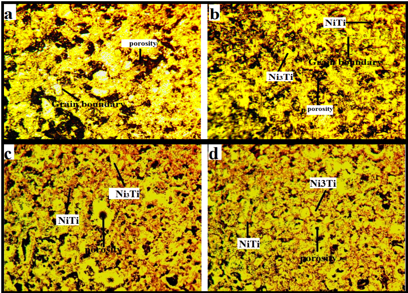
Figure (7): Microstructure for alloys compacted at a: 400 MPa b: 600 MPa
