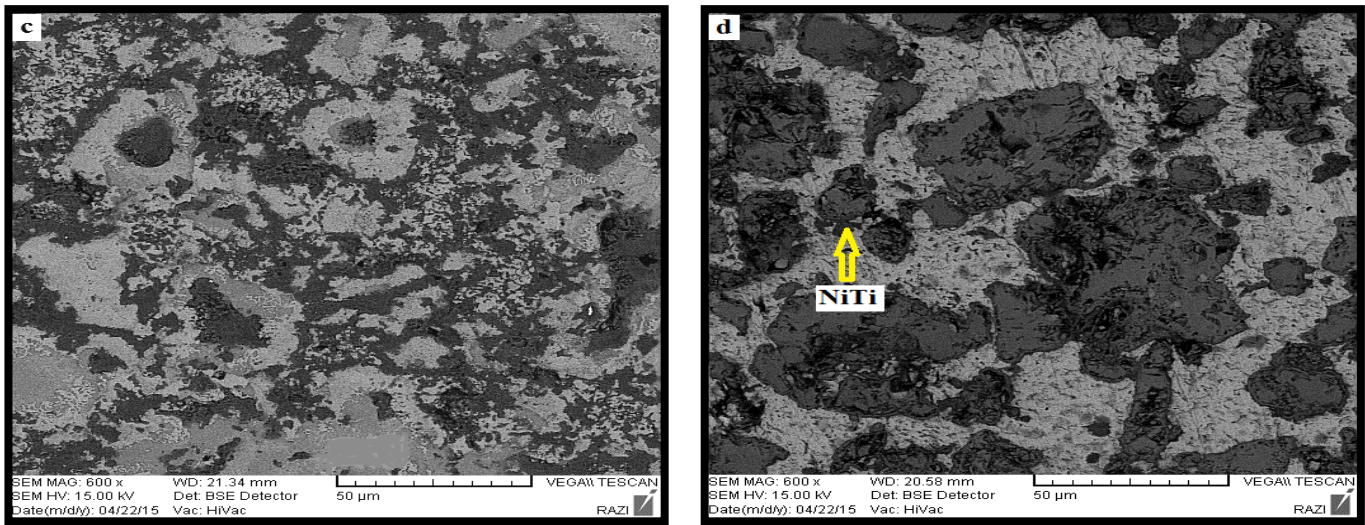
Figure (8): SEM images for etched alloys compacted at a: 400 MPa b: 600 MPa c: 800 MPa d: 900MPa.
