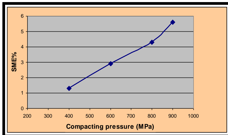
Figure (10): Effect of compacting pressure on SME properties obtained from Brinell Hardness test.
