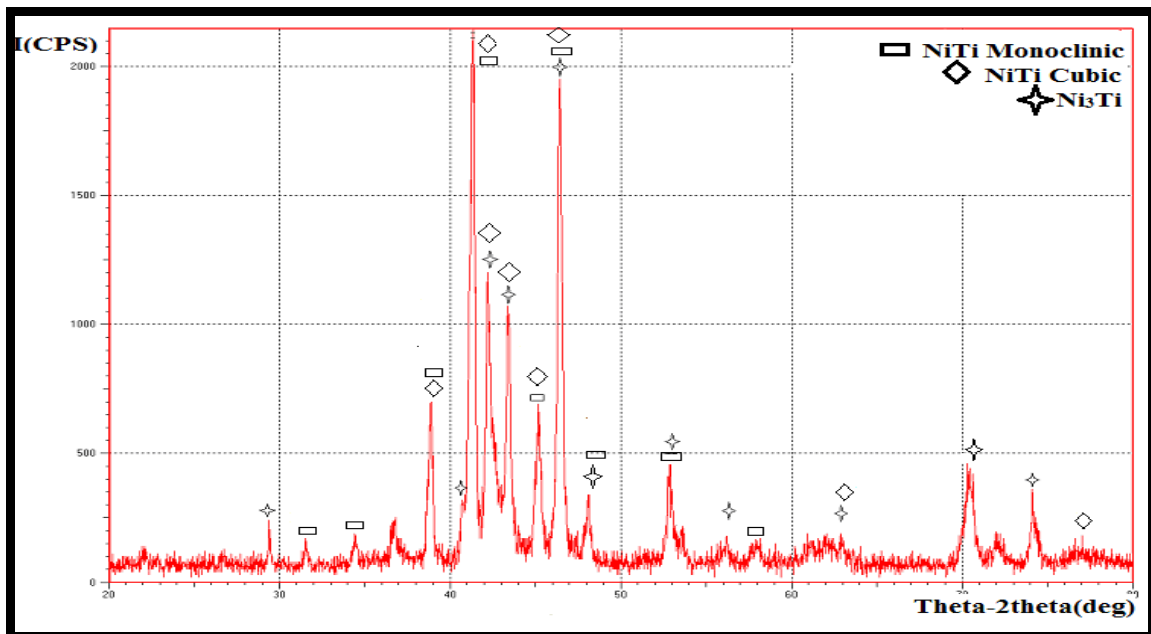
Figure (6): XRD pattern of sample compacted at 800 pressure after sintering.
