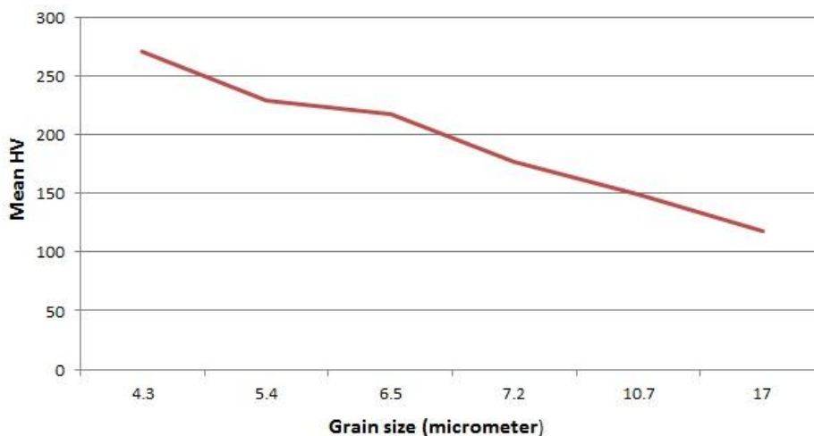
Figure 8: Grains size – mean hardness relationship.
