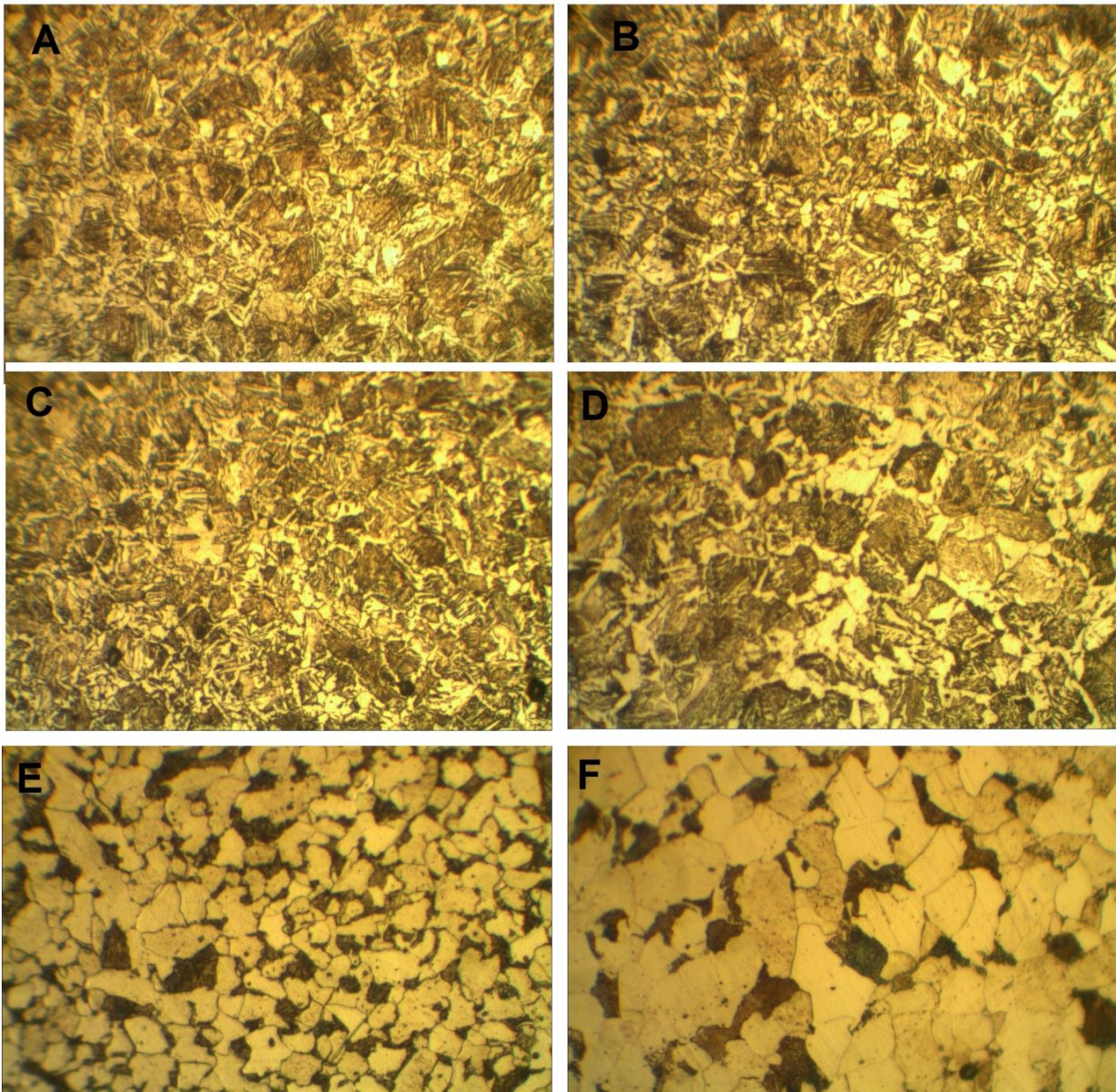
Figure 6: lcy water quenched(A), water quenched(B), oil quenched(C), non-treated(D), air cooled(E), and closed furnace cooled(F).
