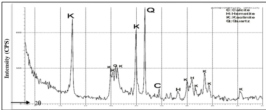
Figure (1). XRD pattern of red kaolin clay.
