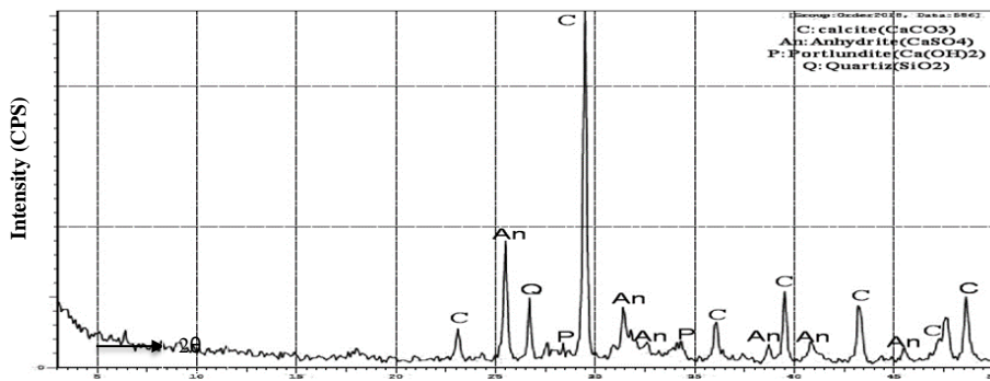
Figure (2). XRD pattern of Kiln dust material.
