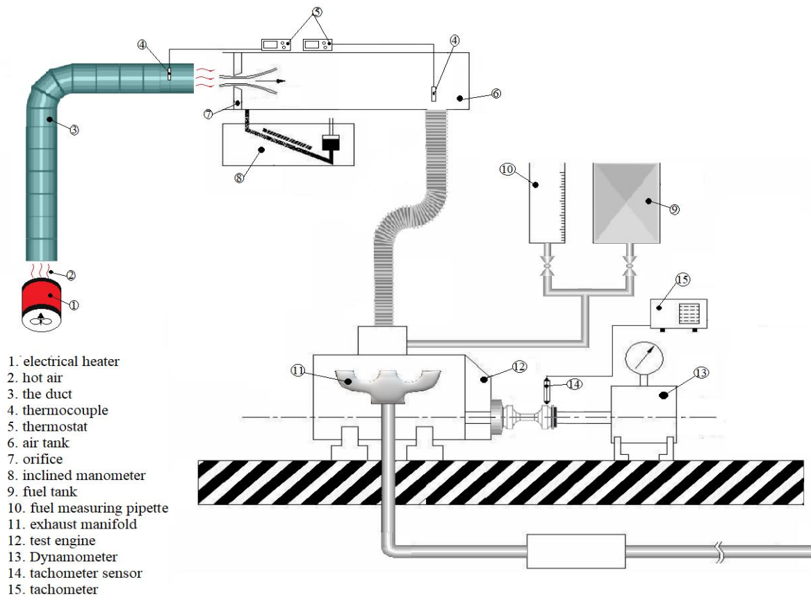
Figure 2. Engine test set up
