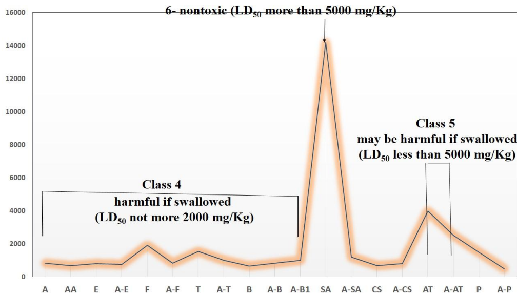
Figure (4). Representative LD 50 and GHS Classes of Toxicity.
