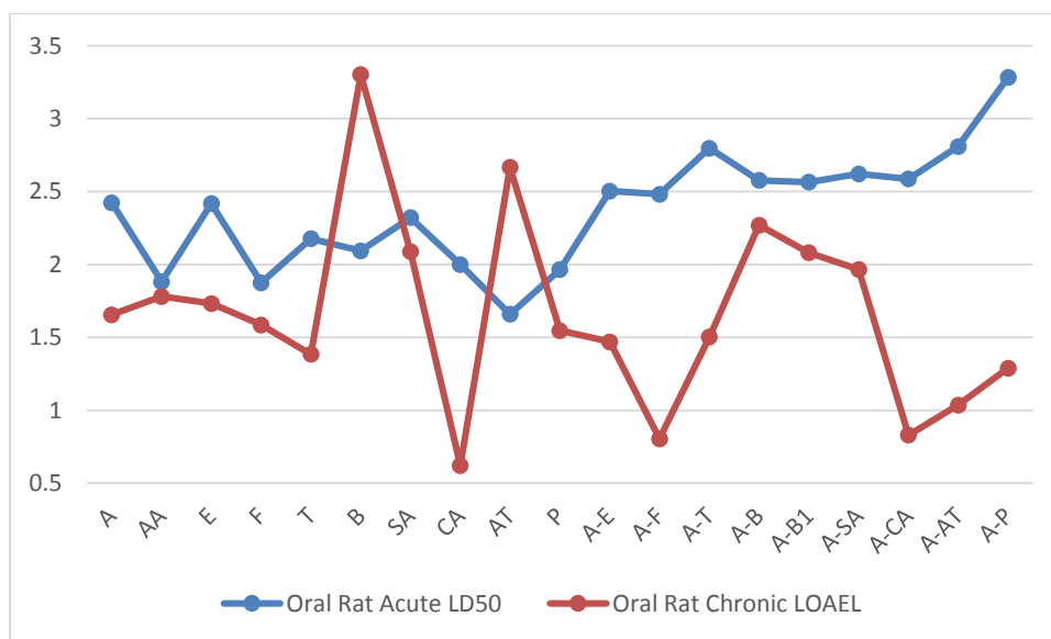
Figure (8). Oral Rat toxicity in acute and chronic terms.
