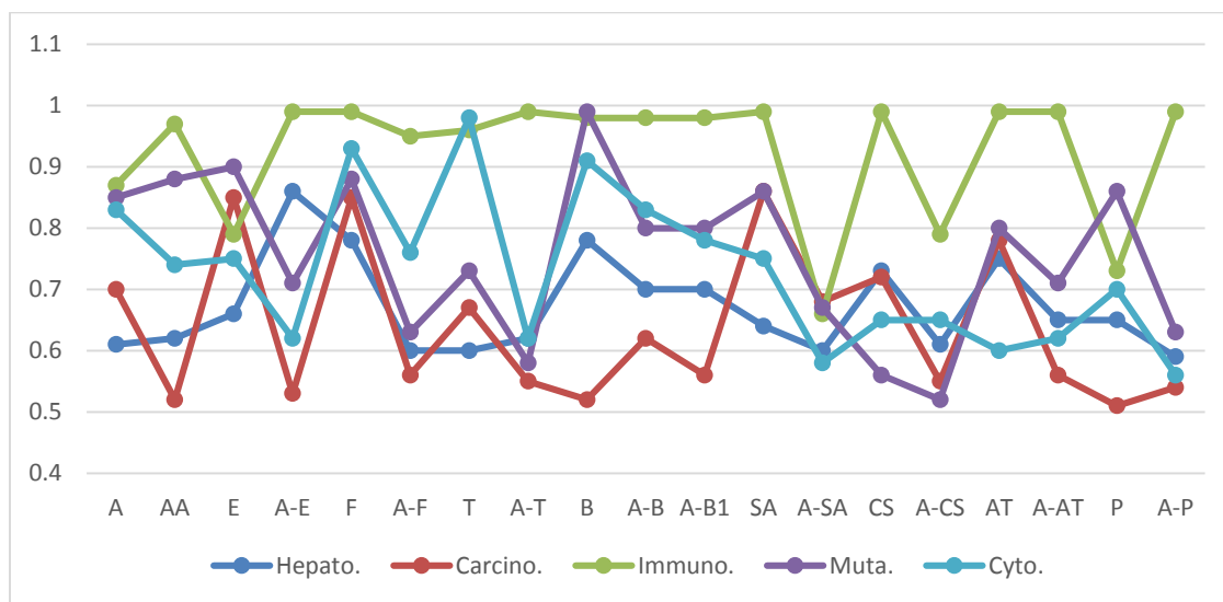
Figure (5). Hepatototoxicity, Carcinogenicity, Immunotoxicity, Mutagenicity, and Cytotoxicity prediction probability.
