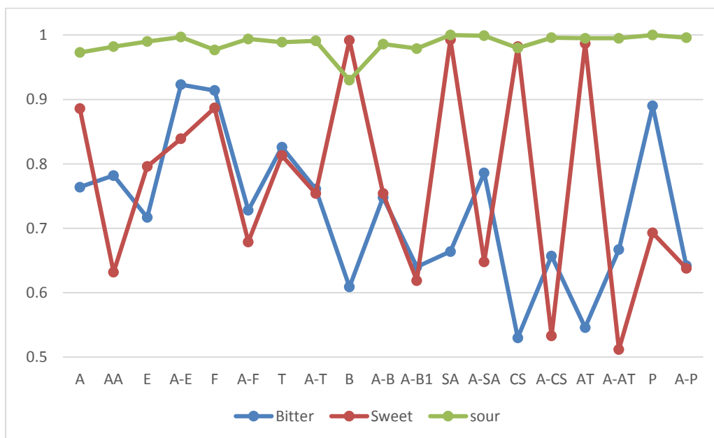
Figure (3). Taste prediction according to http://virtualtaste.charite.de/VirtualTaste/
