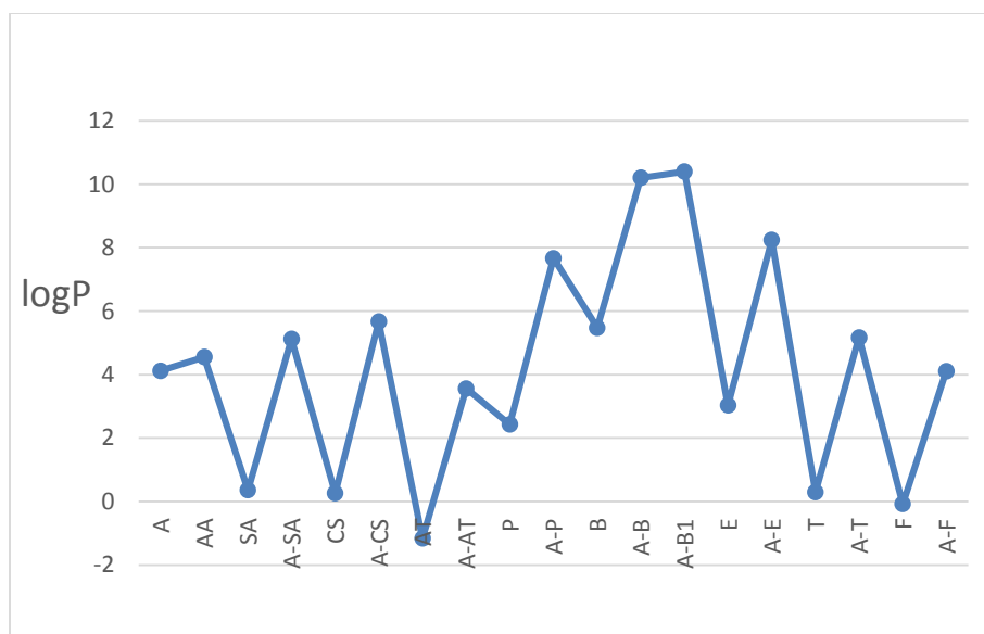
Figure (2). logP of reactants and products.
