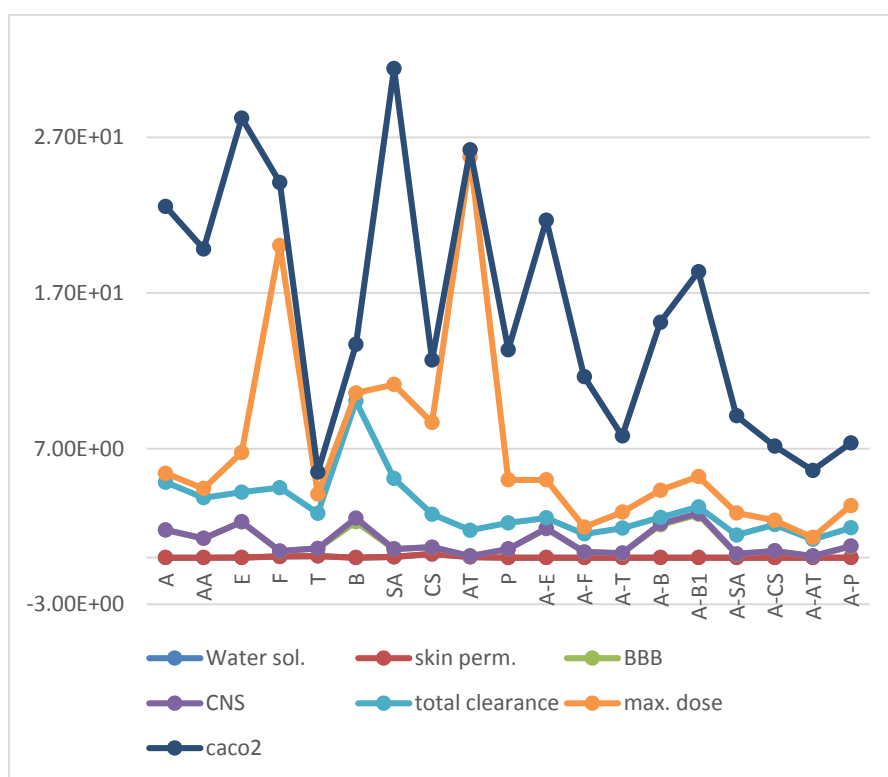
Figure (6). Water solubility, skin permeability, BBB, CNS, Total clearance, maximum dose, and Caco-2 predictors of the reactants and the products.
