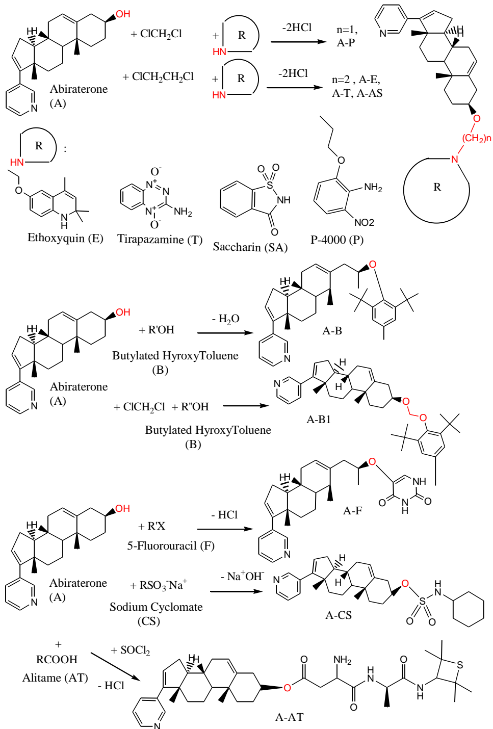
Figure (1). Formation of Hypothetical Abiraterone derivatives.
