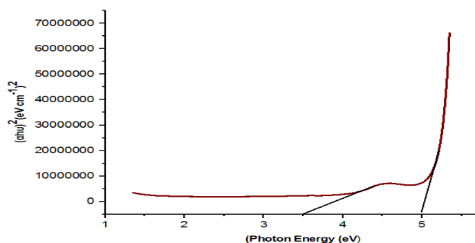
Figure 8 Determination of the optical energy gap of the direct transmission of nanoparticles
