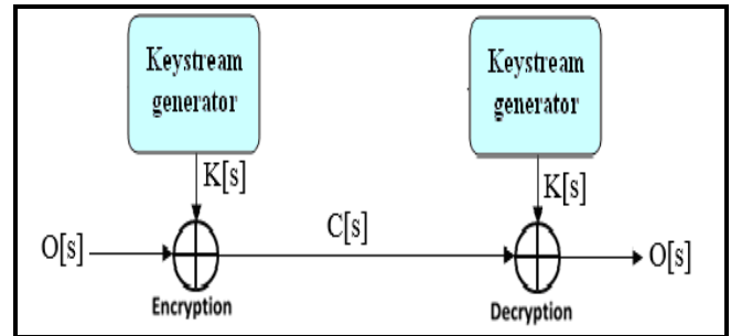
Fig1: Stream Cipher [3]
