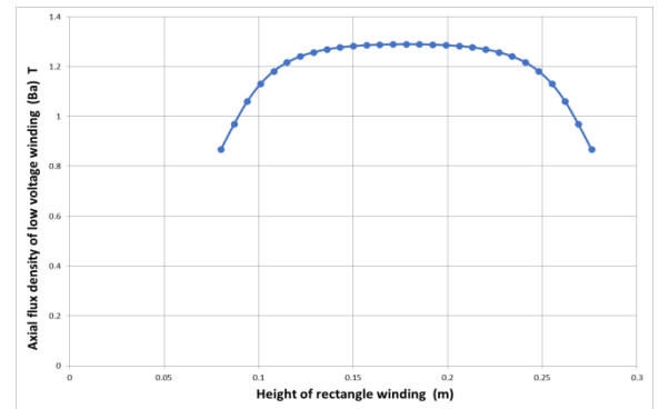
(b) Axial flux distribution along center line of LV coil Figure 21. Axial flux distribution along center line for rectangular windings.
