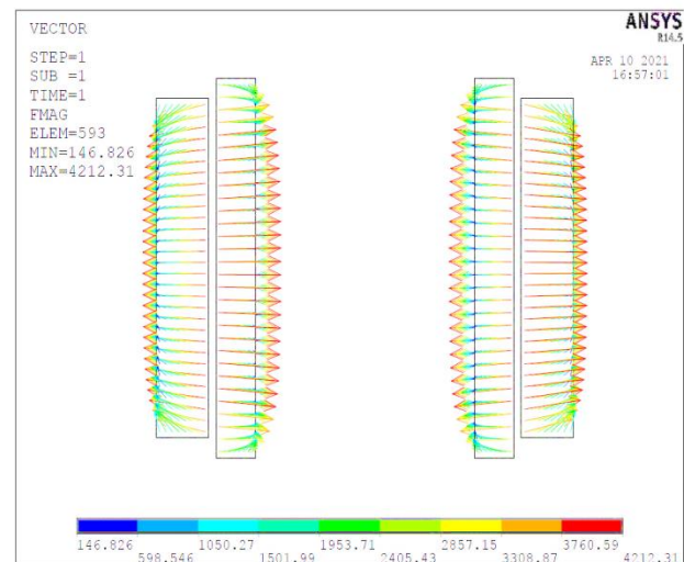
Figure 30. Force vector plot on rectangular coils area.
