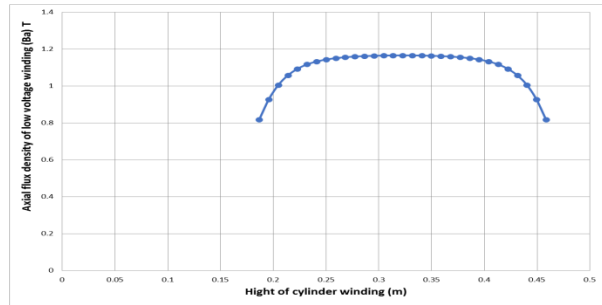
(b) Axial flux distribution along center line of LV coil.
