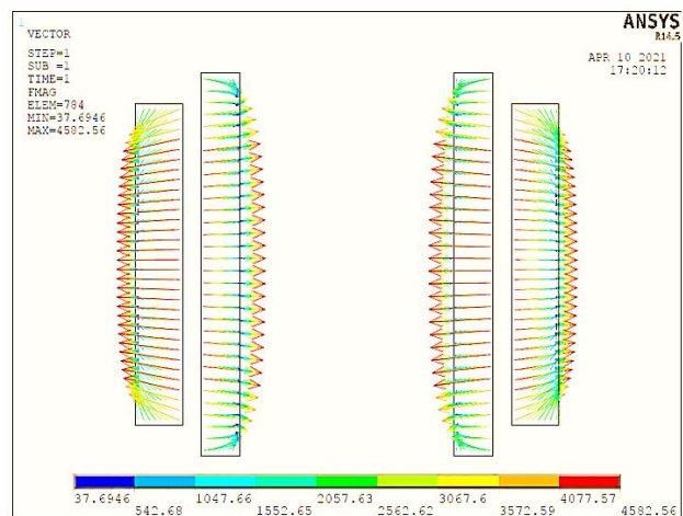
Figure 29. Force vector plot on oval coils area.
