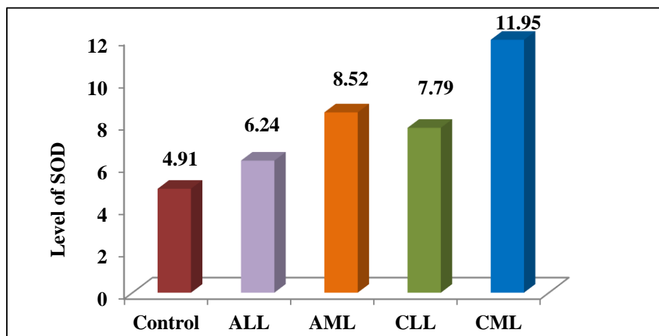
Figure 1: Serum SOD levels in subtypes of leukemia and healthy subjects.
