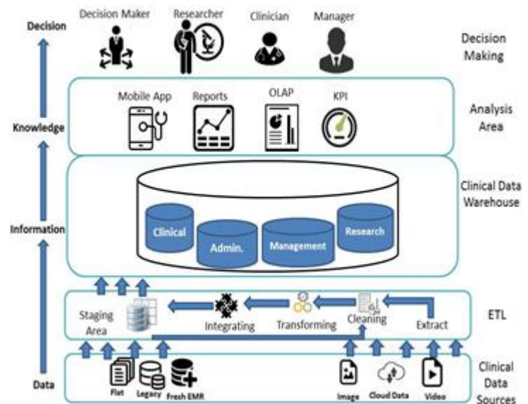
Fig 2: Architecture of CDW
