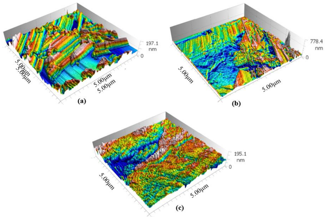
Figure 9: AFM at a magnification (5.00 μm x 5.00 μm) of precursor after chemical activation (a) PPC1, (b) PPC2, and (c) PPC3.
