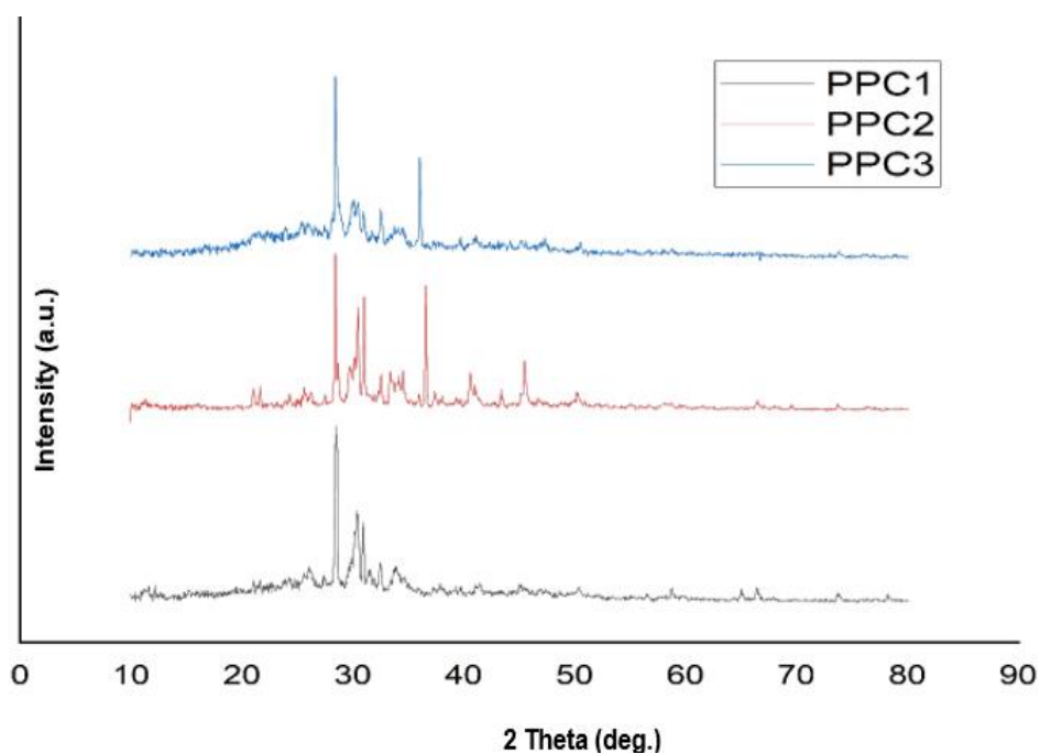
Figure 6: XRD patterns for Physical activation with CO 2 .
