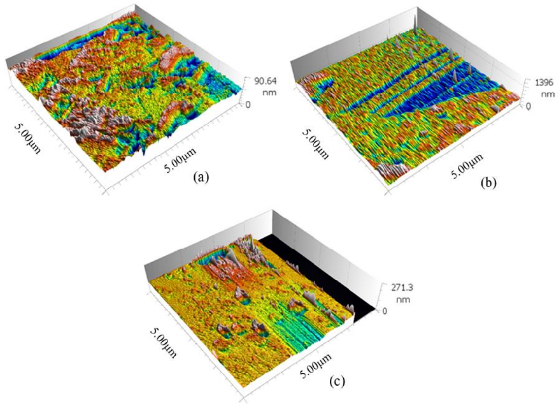
Figure 8: AFM at a magnification (5.00 μm x 5.00 μm) of precursor after chemical activation (a) PPK1, (b) PPK2, and (c) PPK3.
