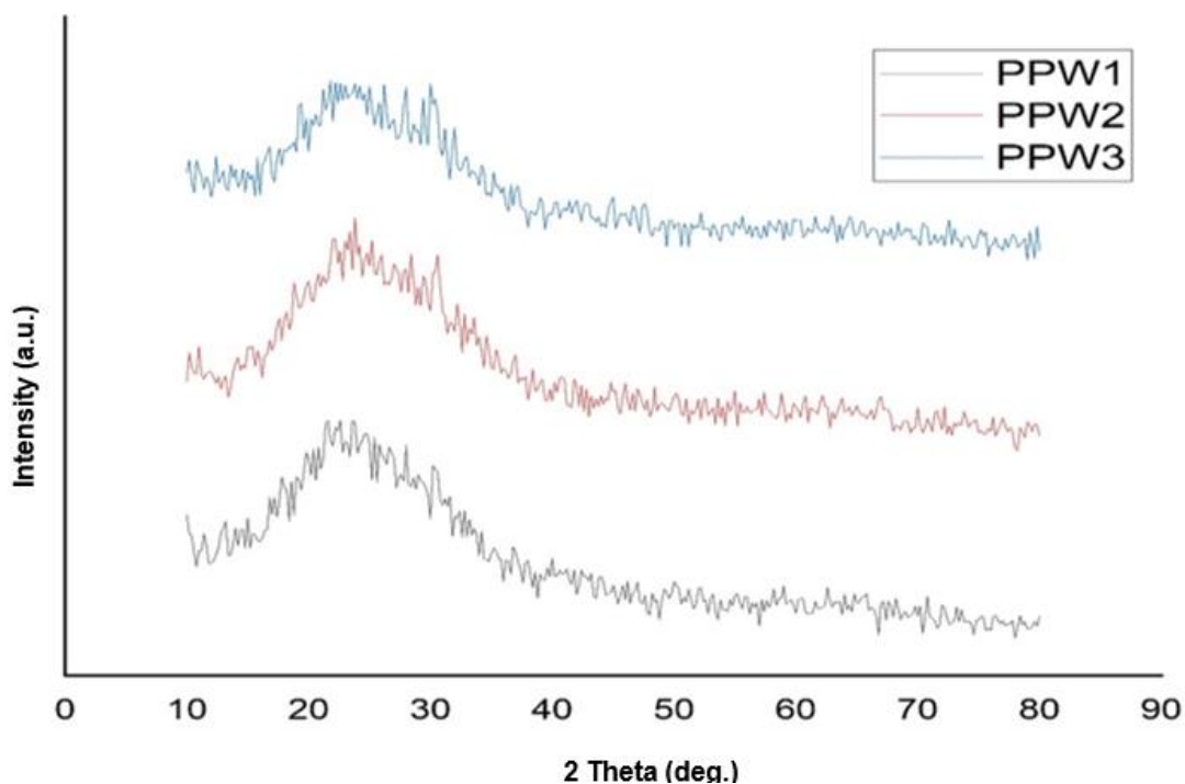
Figure 4: XRD patterns for PPW precursors.
