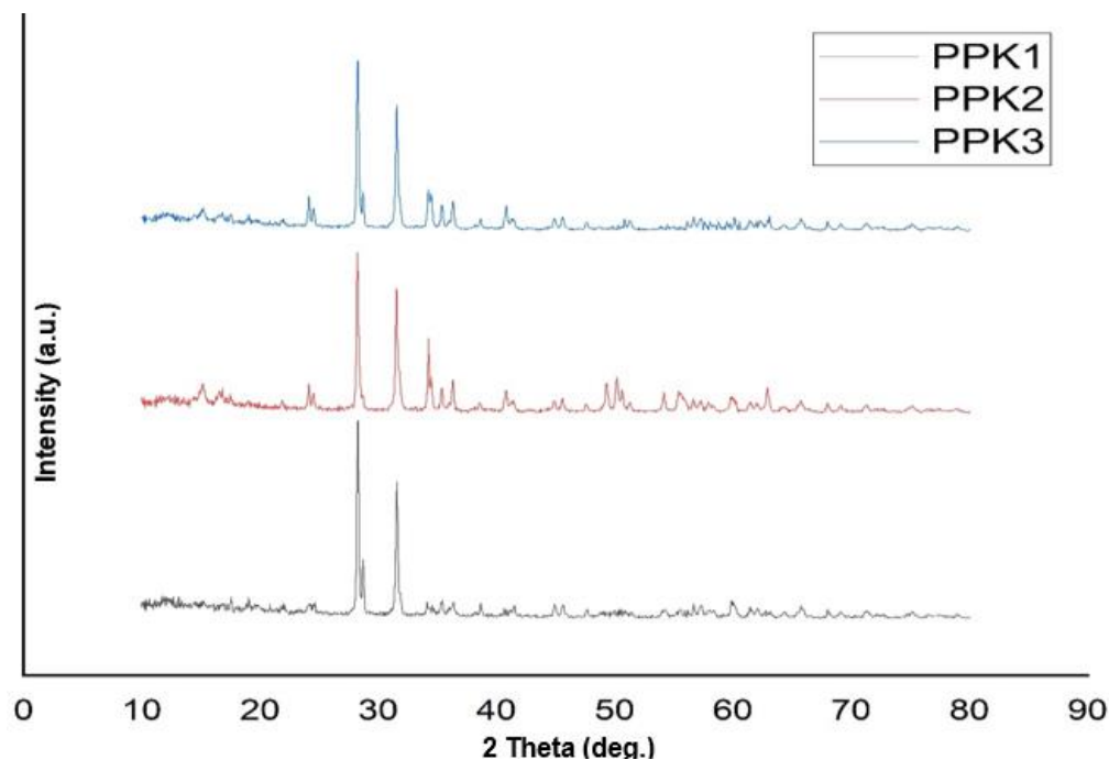
Figure 5: XRD patterns for chemical activation with KOH.
