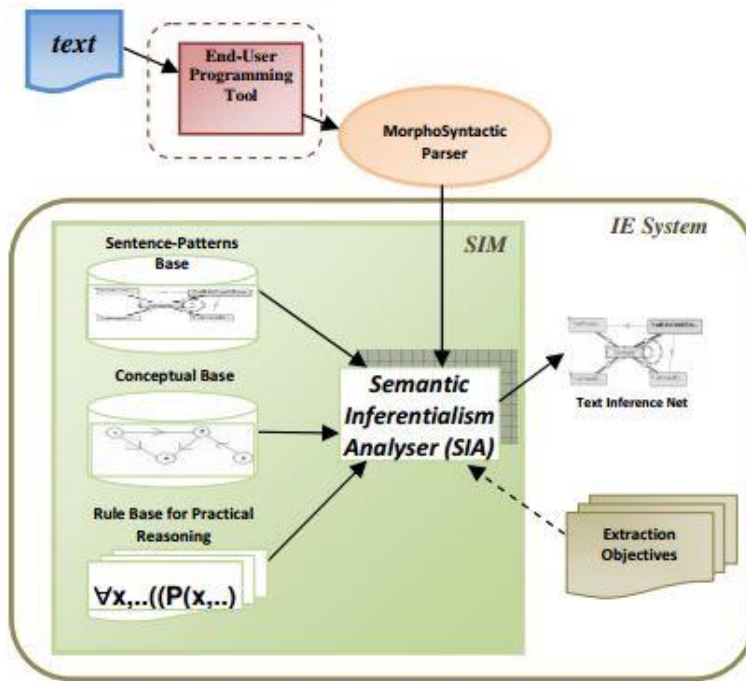
Figure 6. Model architecture.
