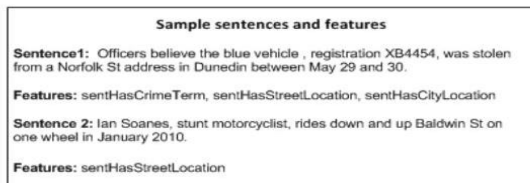
Figure 4. Sample sentences.
