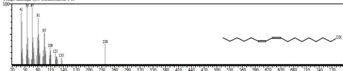
Figure (6): The compound (Z,Z-8,10-Hexadecadien-1-o) diagnosed by GCMS technique
