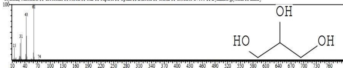
Figure (2): The compound (glycerin) diagnosed by GCM technique
