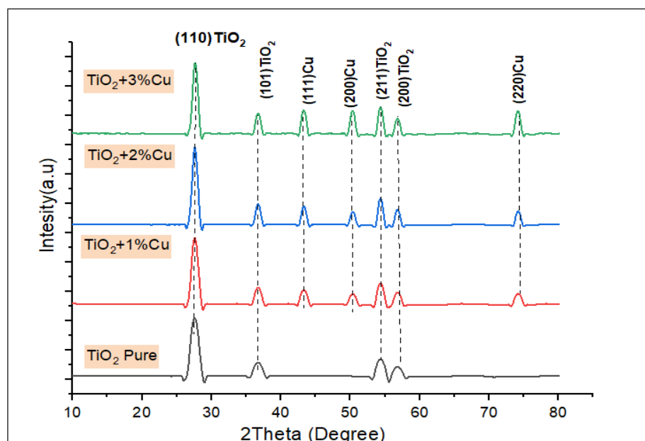
Figure (1). X-ray diffraction of titanium dioxide films doped with copper
