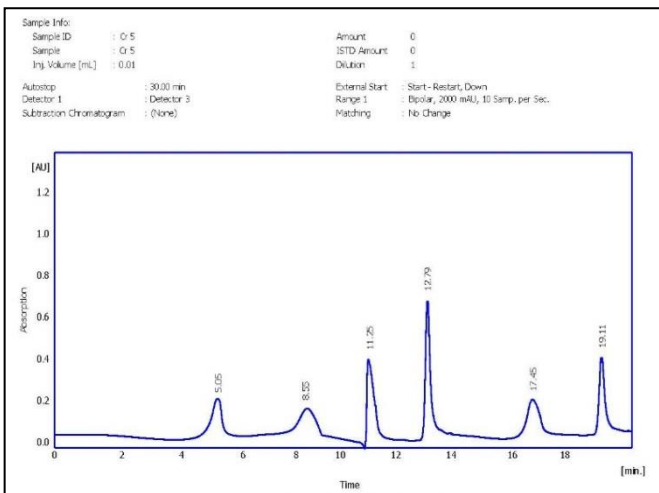
Figure (10): The phenolic compounds form the acid hydrolysis hot aqueous extract (Cr 5 )
