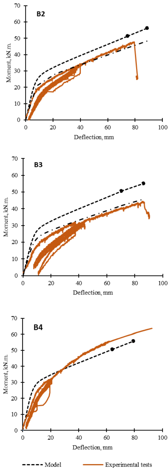
Figure 12. Moment-deflection curves; experimental vs. theoretical prediction ( continued )
