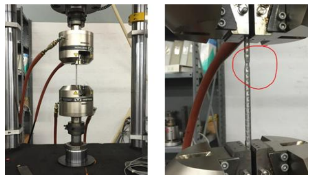
Figure 2. Test setup for steel bars used for stirrups (D5)
