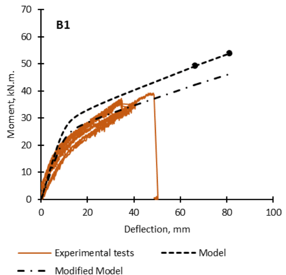
Figure 12. Moment-deflection curves; experimental vs. theoretical prediction
