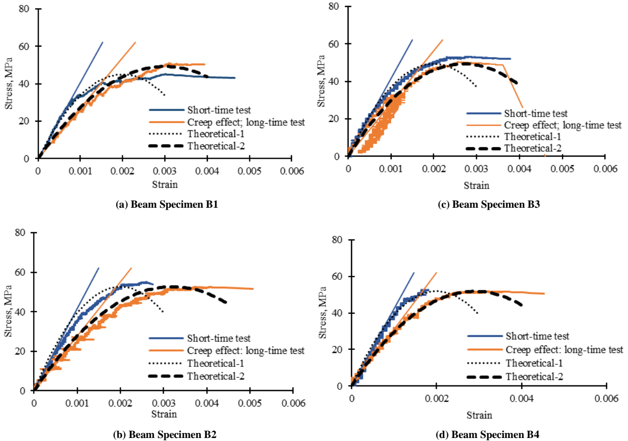
Figure 8. Stress-strain relationship for concrete material considering the creep effect; Theoretical-1 represents the theoretical simulation of the short-time test, and Theoretical-2 represents the theoretical simulation of the long-time test considering the creep effect
