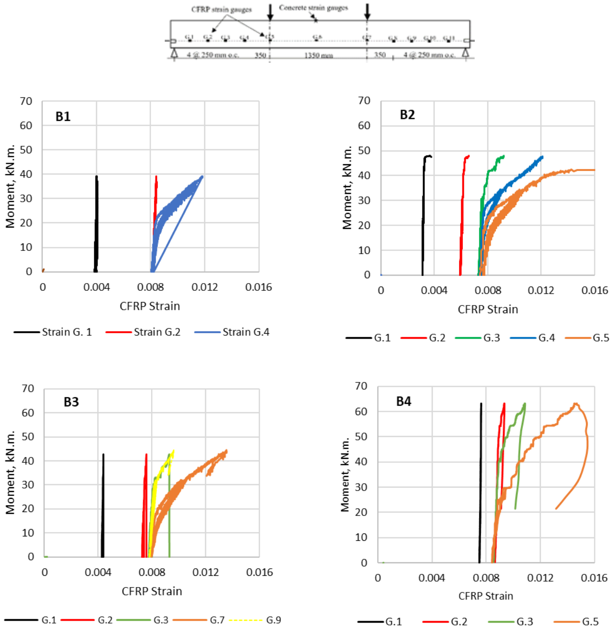
Figure 7. Moment vs. CFRP tensile strain relationship during the flexural test
