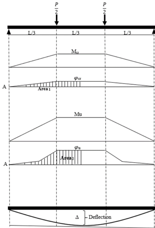
Figure 11. Steps to determine the theoretical mid-span deflection
