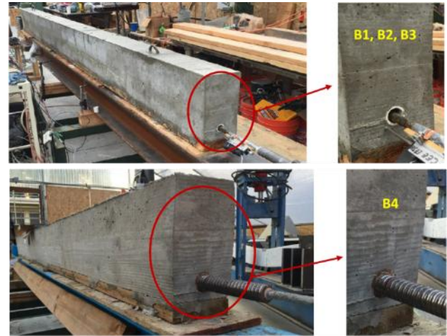
Figure 4. The differences in beam ends for B4 and the other three beam specimens
