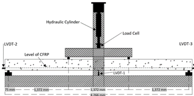
Figure 5. Test setup for beam specimens
