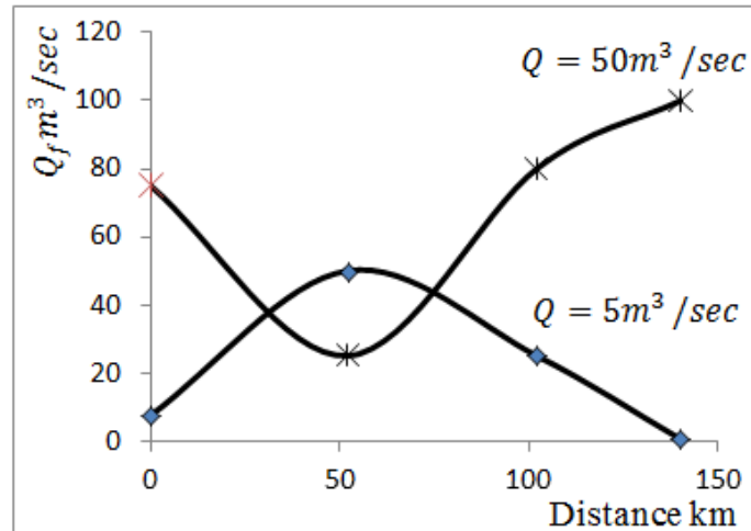
Figure 7. Relation between the distance (km) and Q_f in the River Shatt Al-Arab, at Q : (5, 50) m^3/sec .
