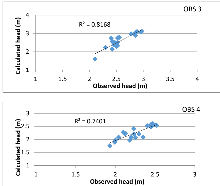
Figure 7. The determination coefficient ( R^2 ) between the observed and calculated heads.
