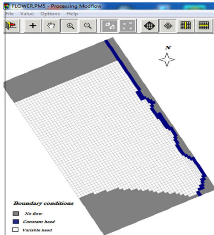
Figure 4. The model grid of the study area.
