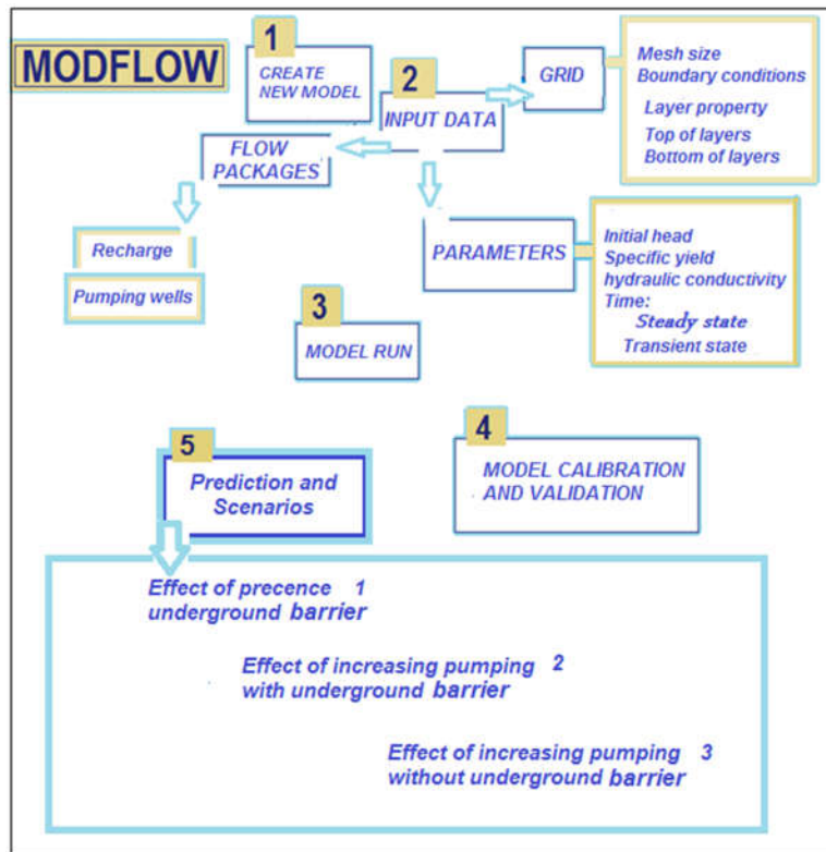
Figure 3. Flow chart of the study area modeling.
