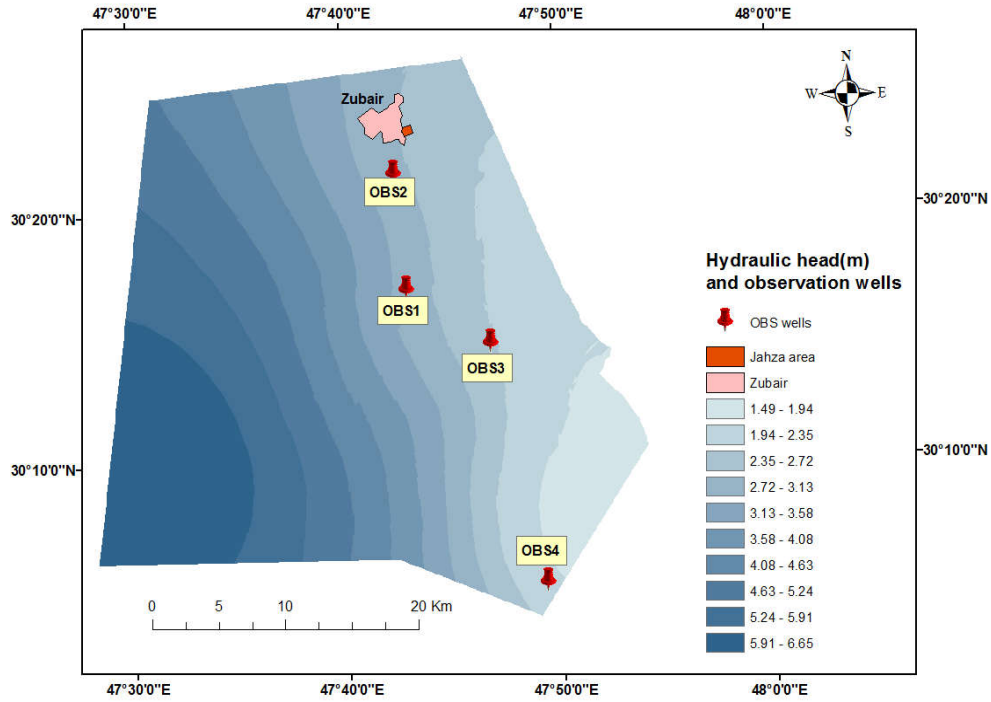
Figure 5. Initial hydraulic head and observation wells.
