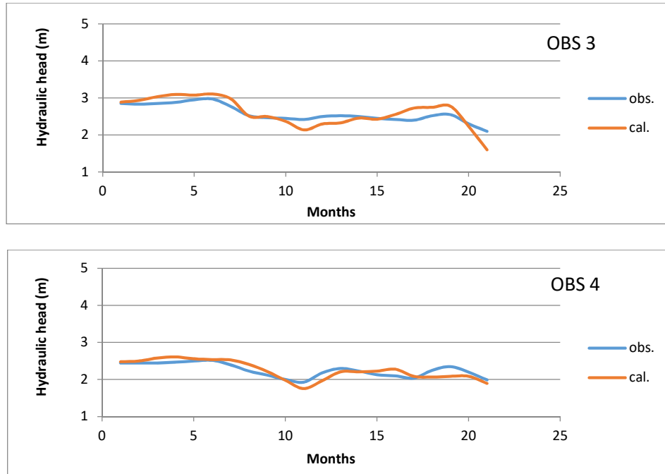
Figure 6. A comparison between the observed and calculated heads.
