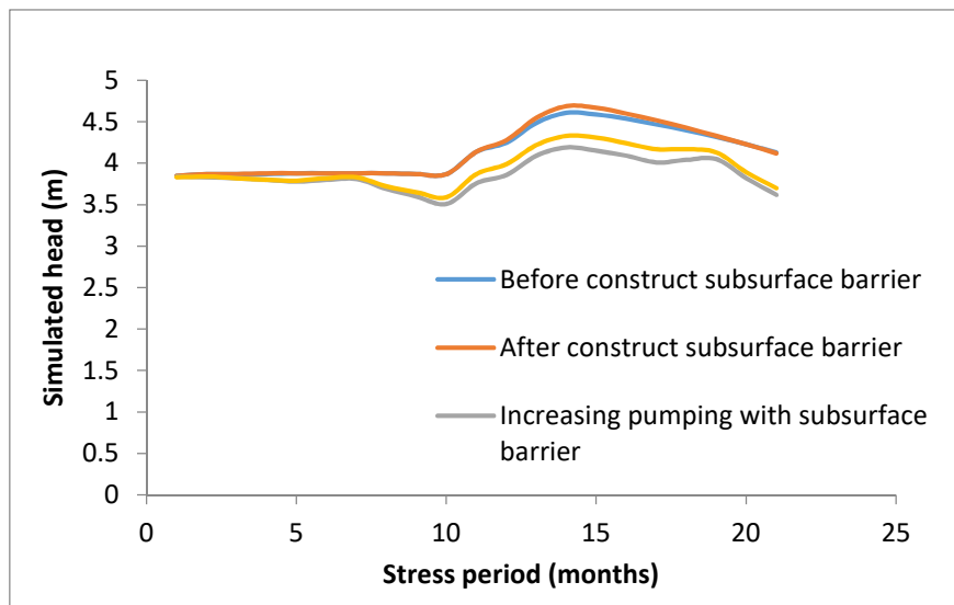
Figure 8. Simulation of levels with and without effect of pumping rate.
