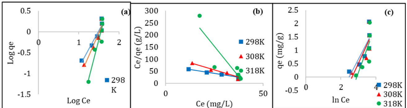
Figure 7. Freundlich (a), Langmuir (b), Temkin (c) isotherm for the adsorption of the MO- dye on the surface of the ES at different temperatures.
