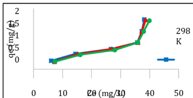
Figure 6. Isotherm of the adsorption process of MO- dye on ES
