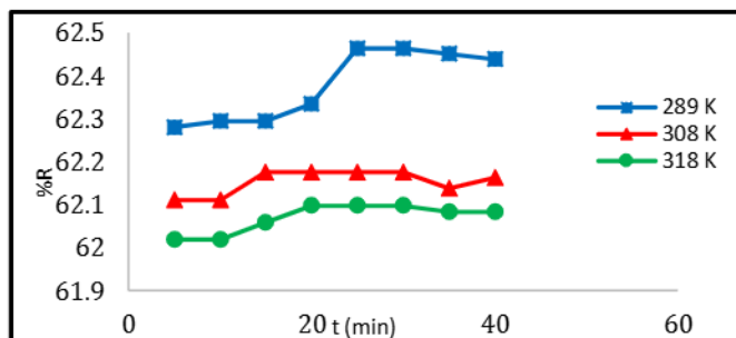
Figure 4. Effect of equilibrium time on the amount of MO - dye adsorbed on the surface of ES.
