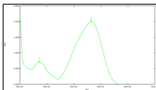
Figure 2. UV-visible absorption spectrum of \text{MO}^- dye.
