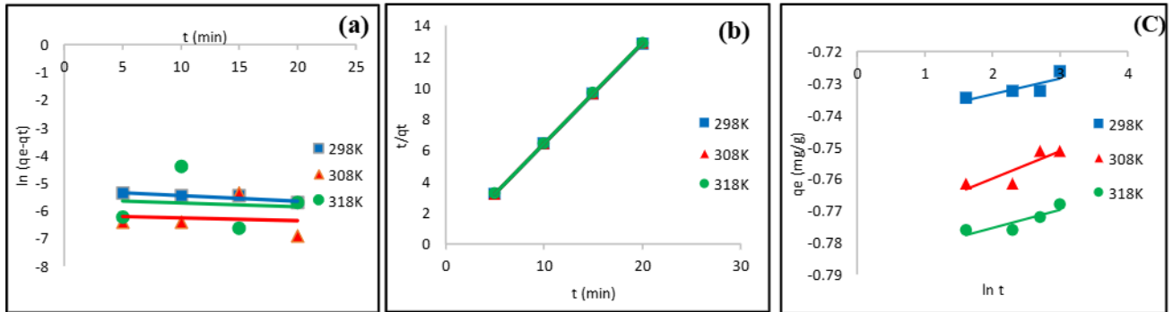
Figure 5. The PFO (a), PSO (b), Elovich (c) kinetic models for the adsorption of the MO- dye on the surface of the ES at different temperatures
