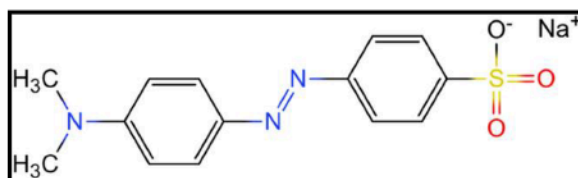
Figure 1. The structural formula of methyl orange.
