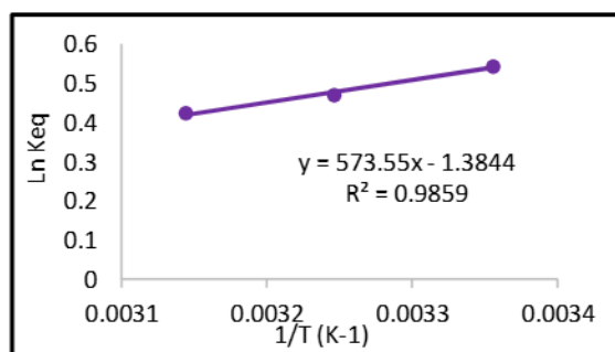
Figure 8. Vant Hof's equation for adsorption of methyl orange dye on the adsorbent surfaces of eggshells .
