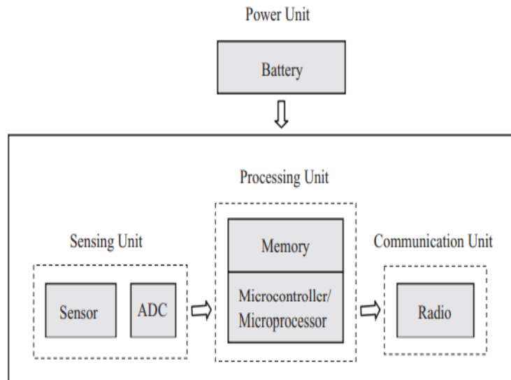
Figure 1: Sensor Node Architecture
