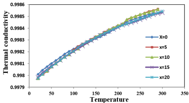
Figure 3. thermal conductivity is represented as a function of temperature of the \text{Se}_{60}\text{Te}_{40-x}\text{Sn}_x glass system ( x = 0, 5, 10, 15, 20 )
