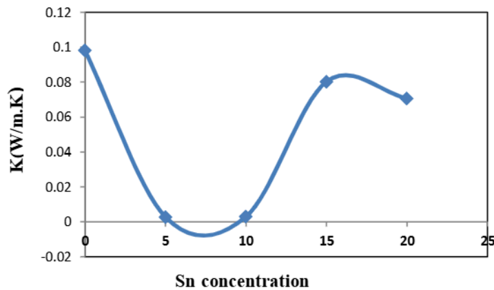
Figure 4. thermal conductivity K as a function of Tin concentration for Se_{60}Te_{40-x}Sn_x alloy
