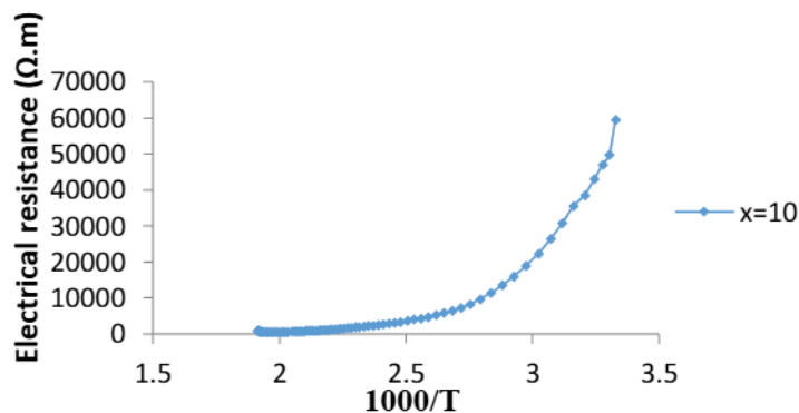
Figure 7. electrical resistance as a function of temperature of of the Se_{60}Te_{40-x}Sn_x glass system ( x = 0, 5, 10, 15, 20 )
