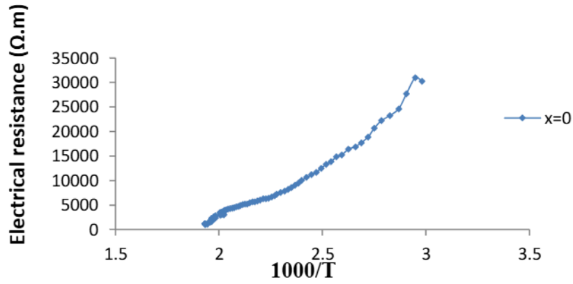
Figure 5. electrical resistance as a function of temperature of of the Se_{60}Te_{40-x}Sn_x glass system ( x = 0, 5, 10, 15, 20 )
