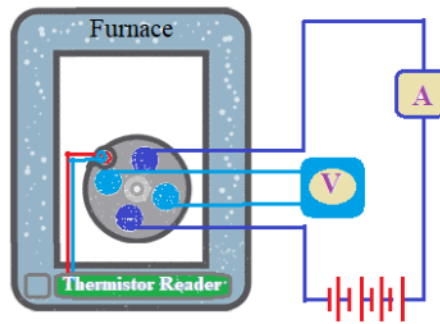
Figure 2. diagram of electrical circuit
