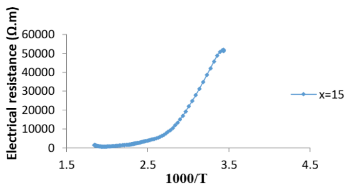
Figure 8. electrical resistance as a function of temperature of of the \text{Se}_{60}\text{Te}_{40-x}\text{Sn}_x glass system ( x = 0, 5, 10, 15, 20 )
