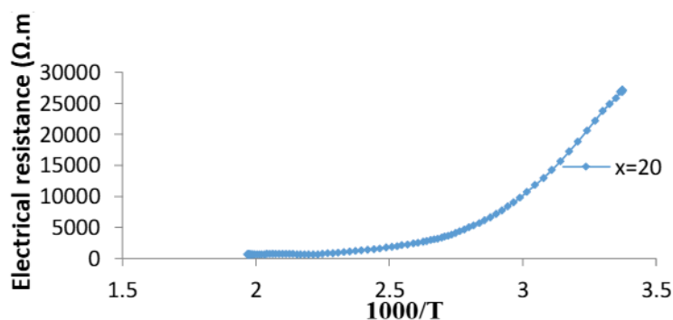
Figure 9. electrical resistance as a function of temperature of of the \text{Se}_{60}\text{Te}_{40-x}\text{Sn}_x glass system ( x = 0, 5, 10, 15, 20 )
