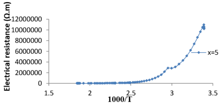
Figure 6. Electrical resistance as a function of temperature of of the Se_{60}Te_{40-x}Sn_x glass system ( x = 0, 5, 10, 15, 20 )
