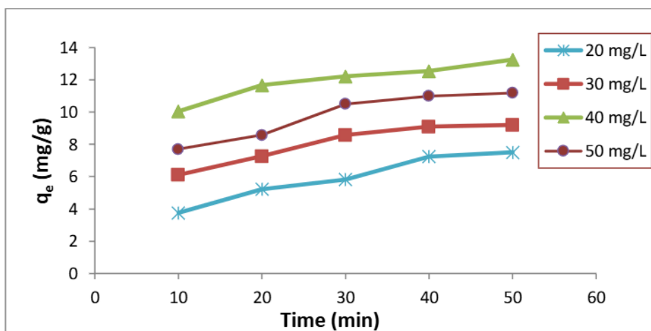
Figure 6. Contact time and initial SY concentration's effect on the adsorption process.
