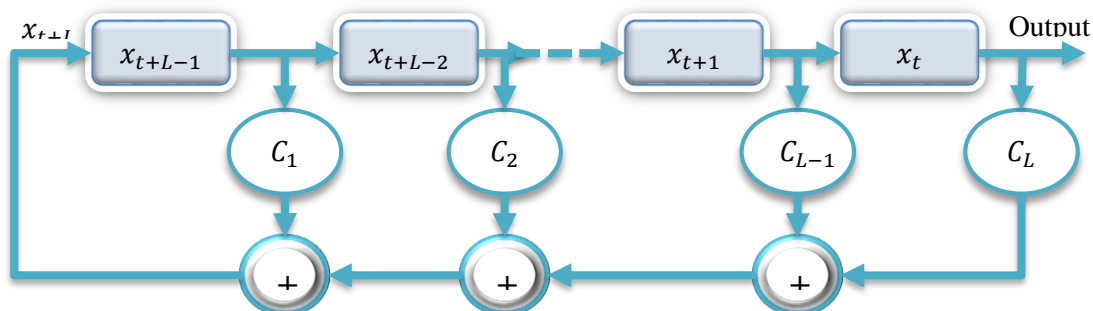
Figure 1. General structure of a LFSR
