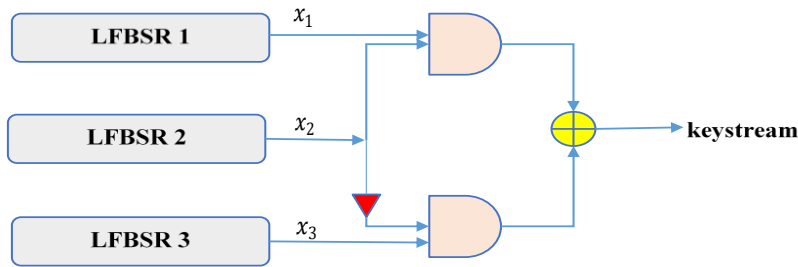
Figure 2. The generator of Geffe
