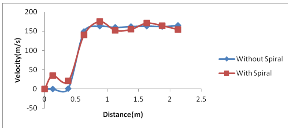
Figure (20): Velocity distribution along cone centerline for inlet air velocity of 0.06 m/s
