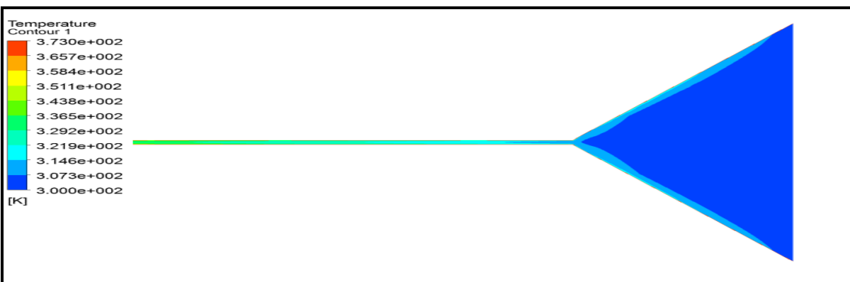
Figure (5): Contour of temperature distribution for smooth cone (without rib) at inlet air velocity 0.04 m/s
