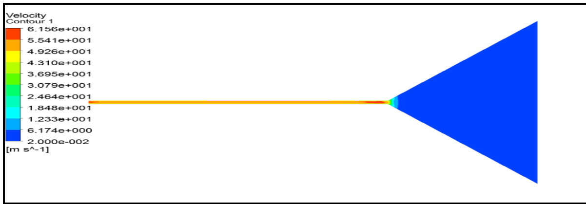
Figure (9): Contour of velocity distribution for smooth cone (without rib) at inlet air velocity 0.02 m/s
