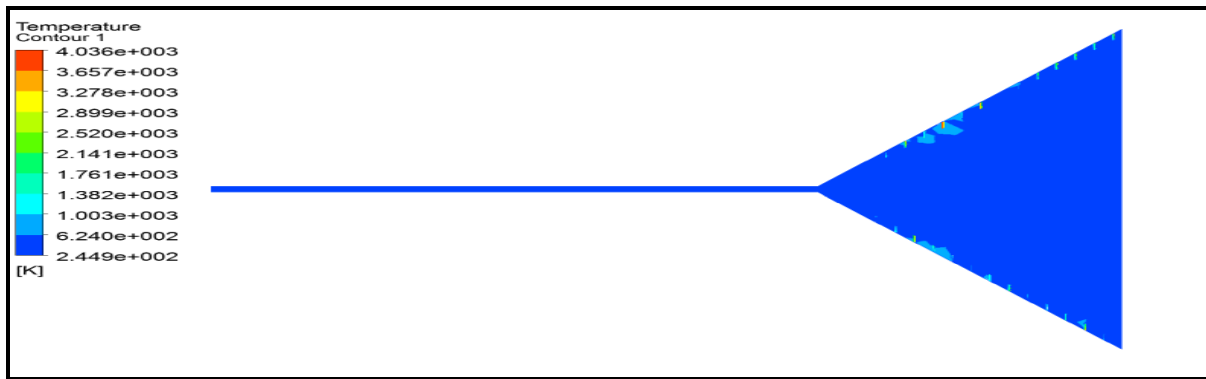
Figure (6): Contour of temperature distribution for cone with spiral square rib at inlet air velocity 0.04 m/s
