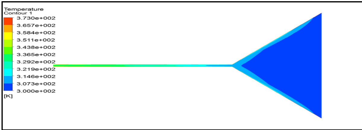
Figure (3): Contour of temperature distribution for smooth cone (without rib) at inlet air velocity 0.02 m/s
