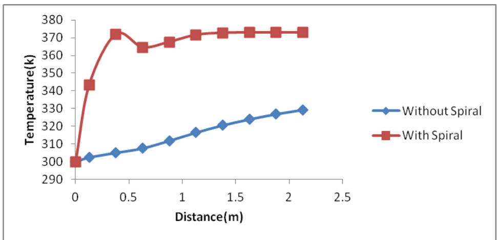
Figure (16): Temperature distribution along cone centerline for inlet air velocity of 0.04 m/s
