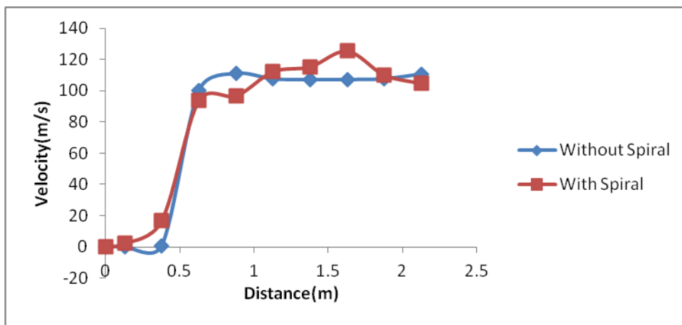
Figure (19): Velocity distribution along cone centerline for inlet air velocity of 0.04 m/s
