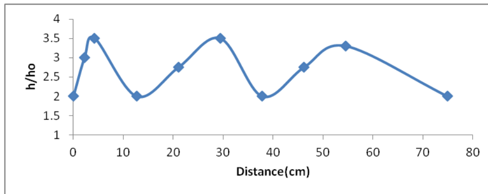
Figure (21): Thermal performance( h/h_o ) for inlet air velocity of 0.02 m/s
