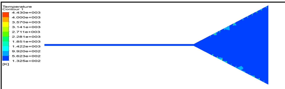
Figure (4): Contour of temperature distribution for cone with spiral square rib at inlet air velocity 0.02 m/s
