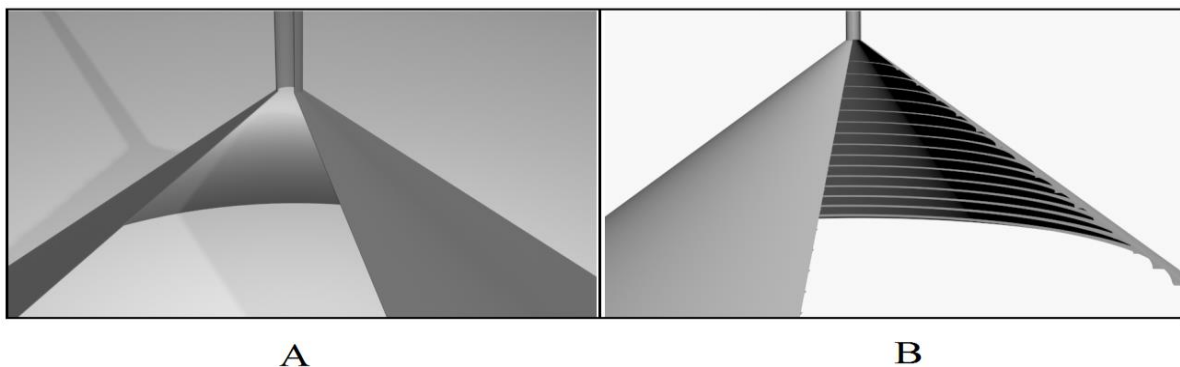
Fig. (1): Simulated conical diffuser : A. smooth cone B. Spiral cone
