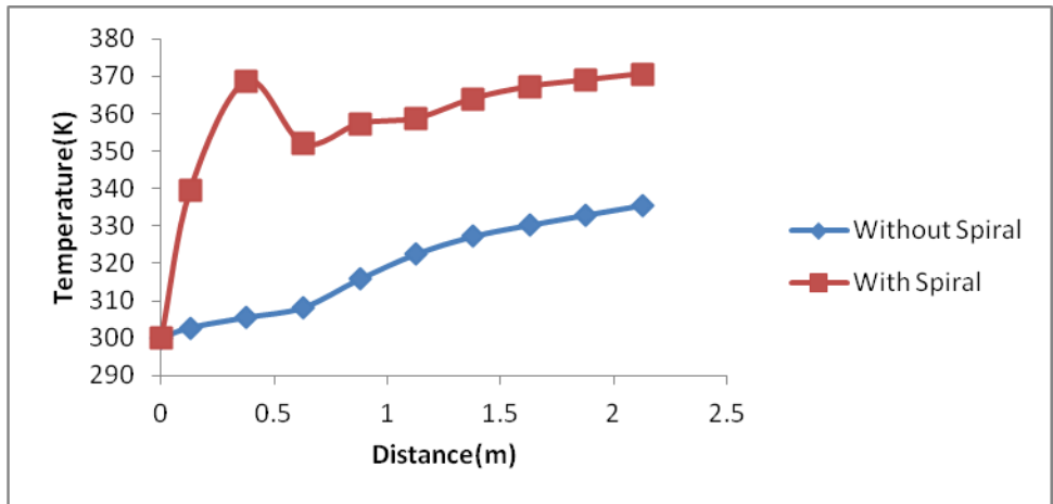
Figure (15): Temperature distribution along cone centerline for inlet air velocity of 0.02 m/s
