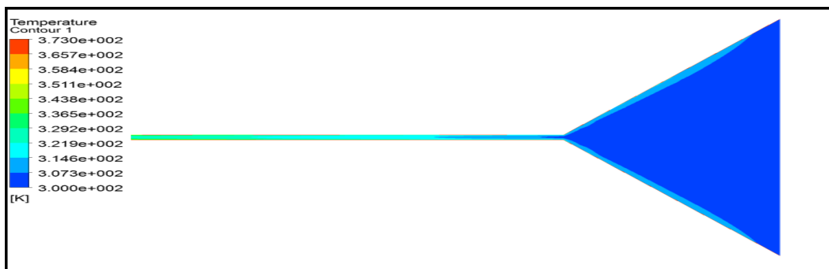
Figure (7): Contour of temperature distribution for smooth cone (without rib) with inlet air velocity of 0.06 m/s
