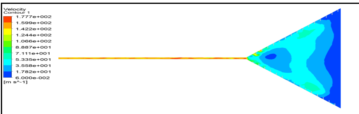
Figure (14): Contour of velocity distribution for cone with spiral square rib at inlet air velocity 0.06 m/s
