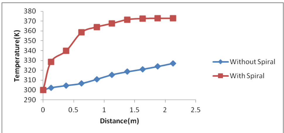
Figure (17): Temperature distribution along cone centerline for inlet air velocity of 0.06 m/s
