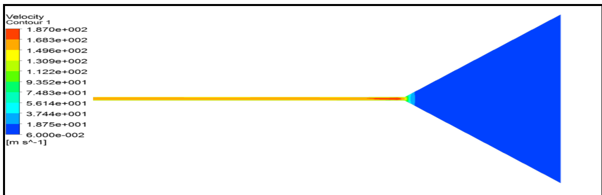
Figure (13): Contour of velocity distribution for smooth cone (without rib) at inlet air velocity 0.06 m/s
