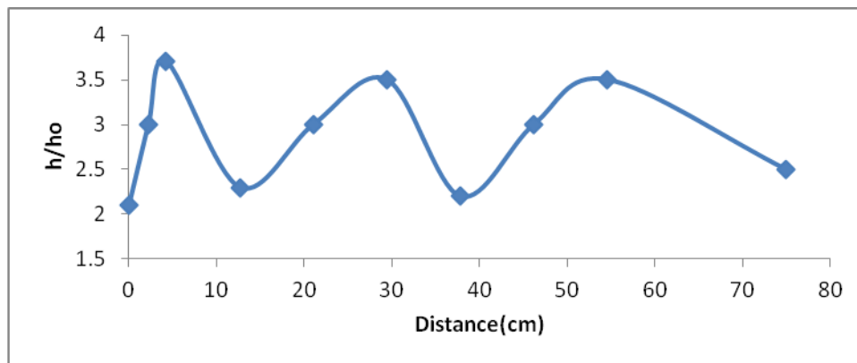
Figure (22): Thermal performance( h/h_o ) for inlet air velocity of 0.04 m/s
