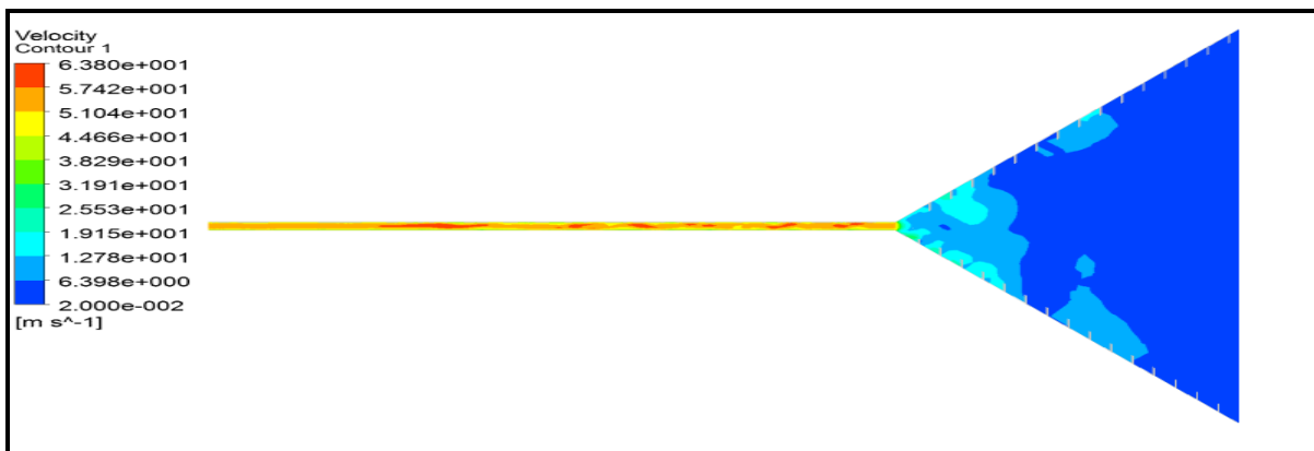
Figure (10): Contour of velocity distribution for cone with spiral square rib at inlet air velocity 0.02 m/s
