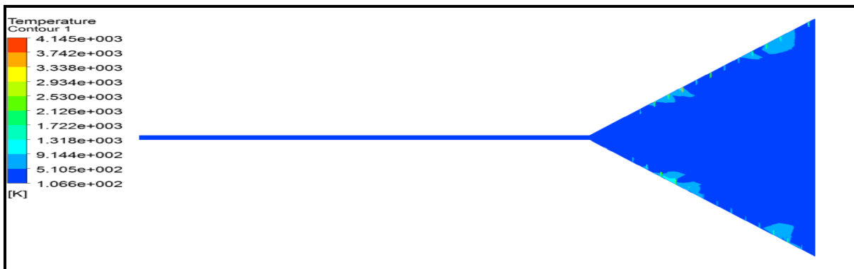
Figure (8): Contour of temperature distribution for cone with spiral square rib at inlet air velocity 0.06 m/s
