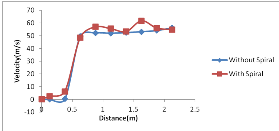
Figure (18): Velocity distribution along cone centerline for inlet air velocity of 0.02 m/s
