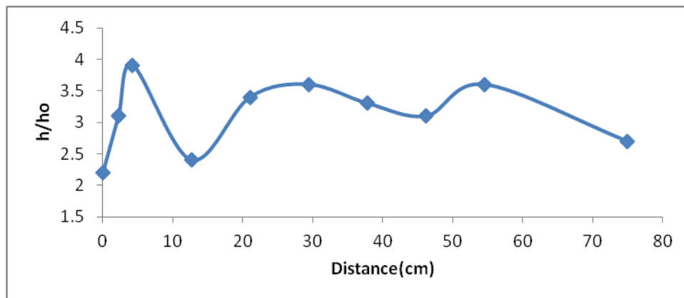
Figure (23): Thermal performance ( h/h_o ) for inlet air velocity of 0.06 m/s
