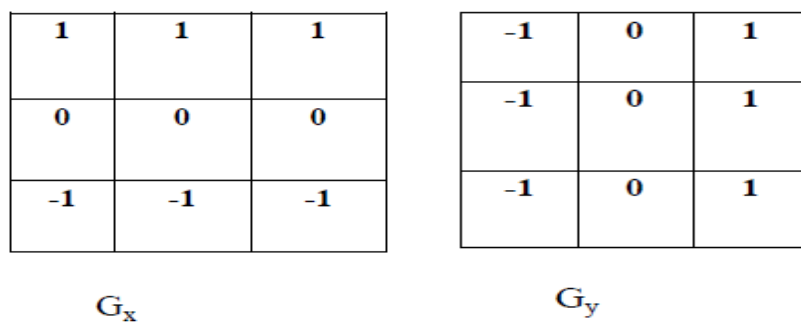
Figure 1: Prewitt Operator
