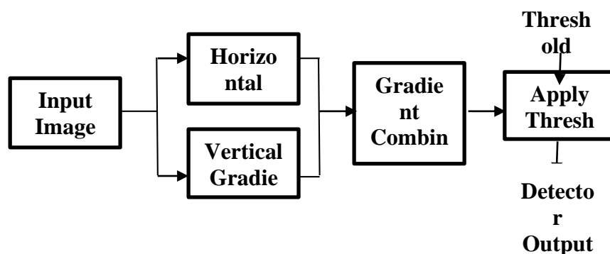
Figure 2: Process of Prewitt Edge Detection
