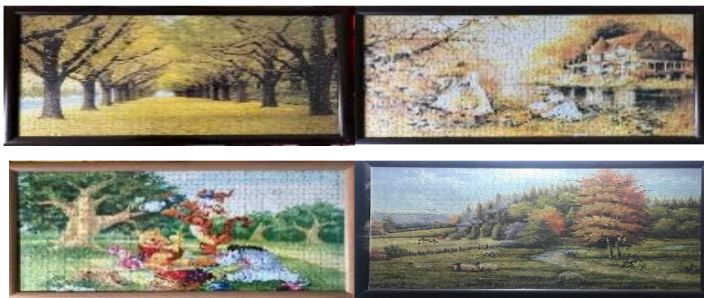
Figure 3: Dataset Samples
