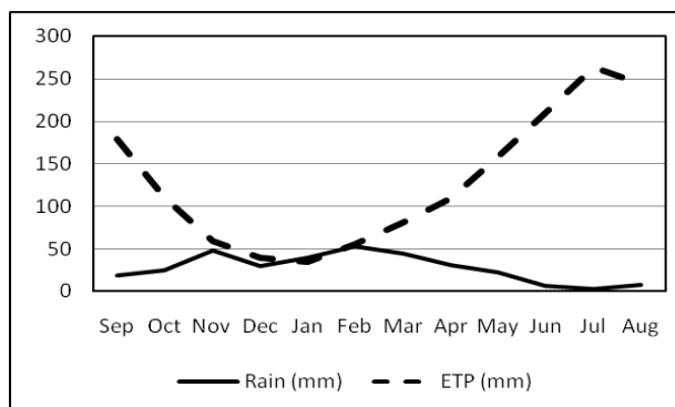
FIGURE 2. Climatic characteristics.
