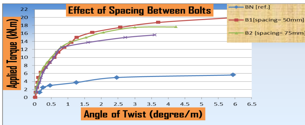
Figure (10): Torque–Twist Behavior of Composite Concrete-Steel Beams
