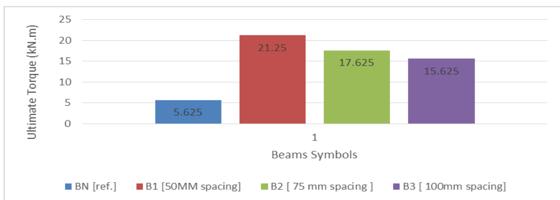
Figure (9): Load carrying capacity of the tested beams
