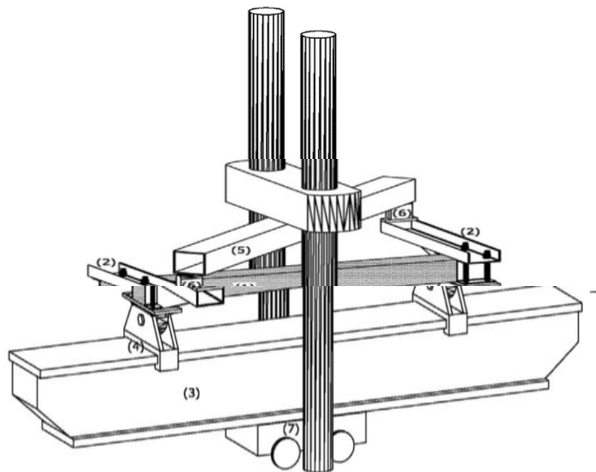
Fig. (5) clamping loading frame
