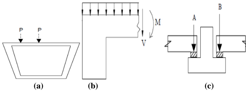
Figure (1): Examples of torsion in structural members [3]
