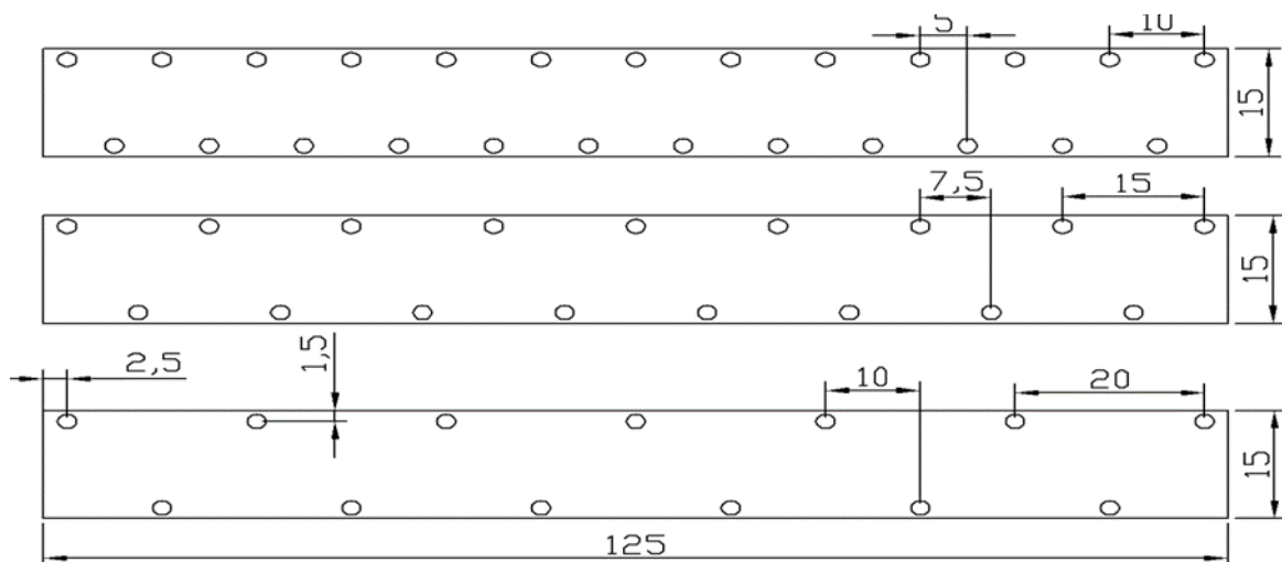
Figure (2) Typical Bolts Distribution of the Steel Plates [all dimensions in centimeter (cm)]
