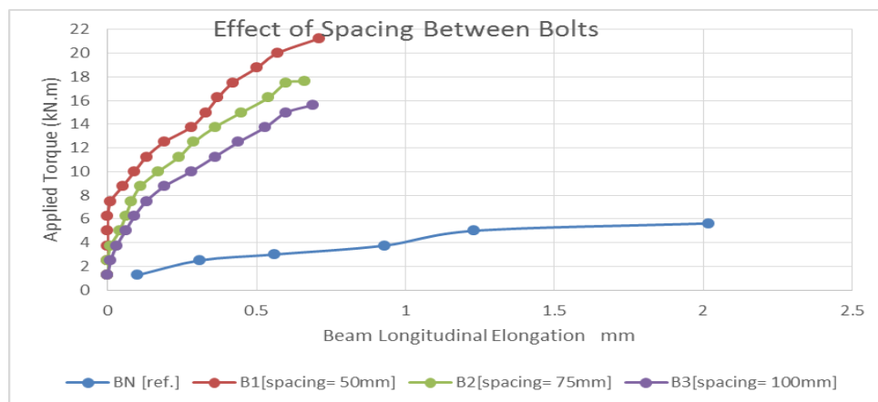
Figure (11): Torque– Longitudinal Elongation Behavior of Composite Concrete-Steel Beams
