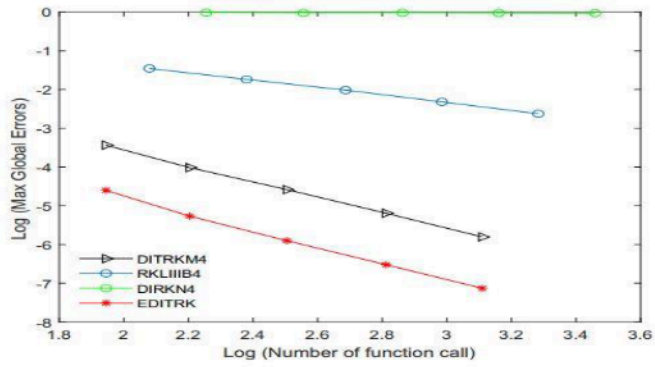
Figure 2. Accuracy curve for EDITRK4, DITRKM4, RKLIIIB4, and DIRKN4 with h = 0.1, 0.05, 0.025, 0.00125, and 0.00625 for the problem 2.
