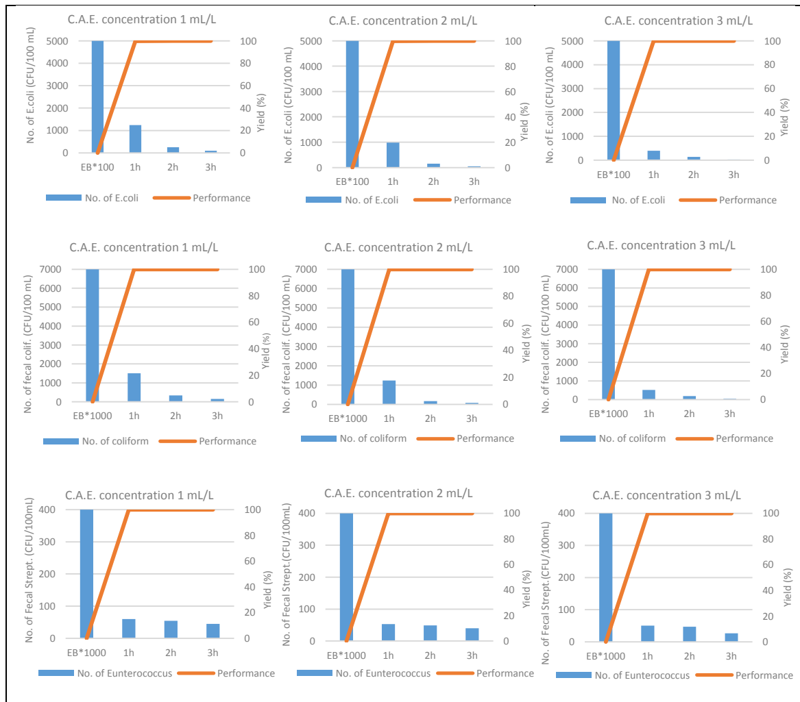
FIGURE 1. Effect of C.A.E. on the elimination of indicator germs of fecal contamination.
