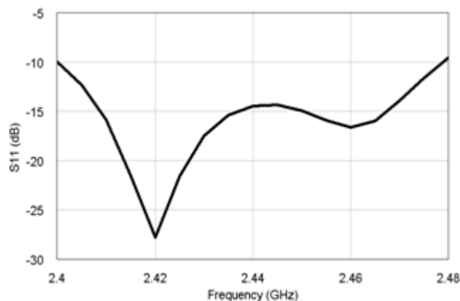
Fig.2 The calculated input returns loss for the modeled patch
