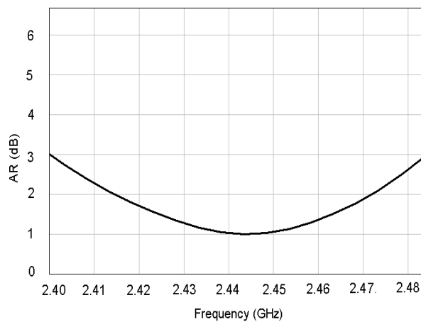
Fig.4 The computed axial ratios around the IEEE802.11b/g frequency, for the proposed antenna.
