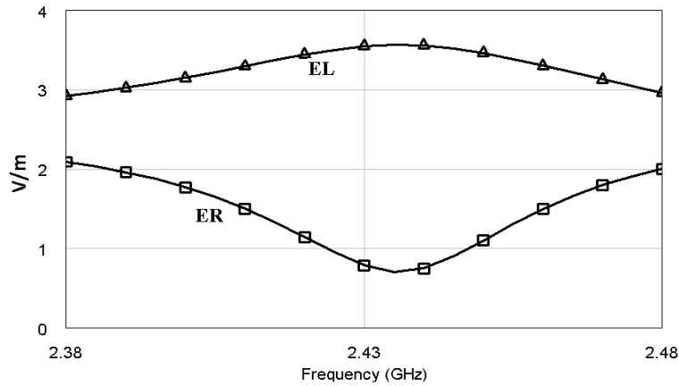
Fig.3 The computed far electric field intensity left hand and right hand circular polarization in broadside direction, of the proposed
