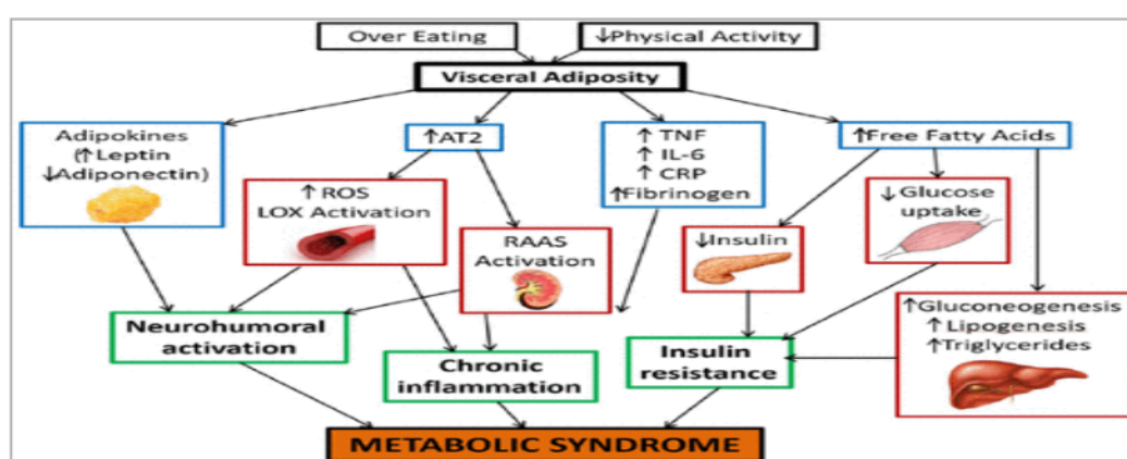
Figure 1. Mechanisms of metabolic pathophysiology. C-Reactive Protein (CRP), interleukin 6, IL-6, ROS, reactive oxygen species; TNF, tumor necroses factor (At2, angiotensin II type 2 receptor; RAAS, Renin-angiotensin-aldosterone systems; Reactive oxygen species (ROS)). [27].
