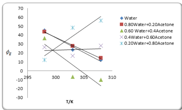
Figure (2): a plot of ( \phi_E ) against (T) fo sodium acetate in A) water B)20% Water+Acetone C) 40% Water+Acetone D) 60% Water+Acetone E) 80% Water+Acetone mixtures at 298.15K, 303.15K and 308.15 K
