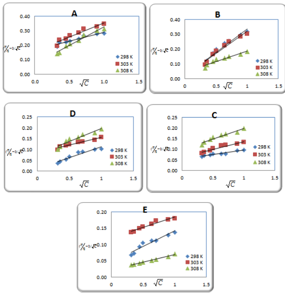
Figure (3):Plots of (\eta-1)/\sqrt{c} ( L^{3/2}\cdot mol^{-1/2} ) vs \sqrt{c} ( mol^{1/2}\cdot L^{3/2} ) for sodium acetate in A) water B) 20% Water+Acetone C) 40% Water+Acetone D) 60% Water+Acetone E) 80% Water+Acetone mixtures at different temperatures
