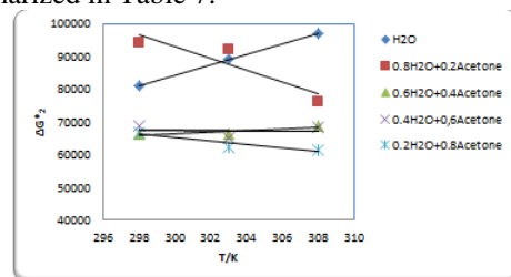
Figure (4): Plots of (\Delta G_2^*) vs (T) for sodium acetate in A) water B) 20% Water+Acetone C) 40% Water+Acetone D) 60% Water+Acetone E) 80% Water+Acetone mixtures at different temperatures
