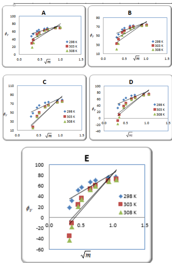
Figure 1: A plot of apparent molal volume ( \phi_v ) against ( \sqrt{m} ) of sodium acetate in A) water B) 20% Water+Acetone C) 40% Water+Acetone D) 60% Water+Acetone E) 80% Water+Acetone mixtures at different temperatures.
