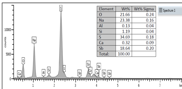
Fig4.: The EDAX is curved to the \text{Sb}_2\text{S}_3 film at deposition temperature 50^\circ\text{C}
