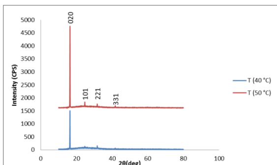
Fig. 2: X-ray diffraction of \text{Sb}_2\text{S}_3 thin films at (40,50) °C.
