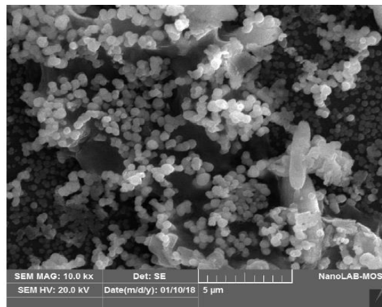
Fig.3: Scanning electron microscopy of \text{Sb}_2\text{S}_3 thin films at deposition temperature 50^\circ\text{C} .
