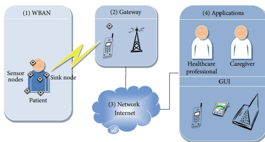
Figure 1:WBAN Architecture
