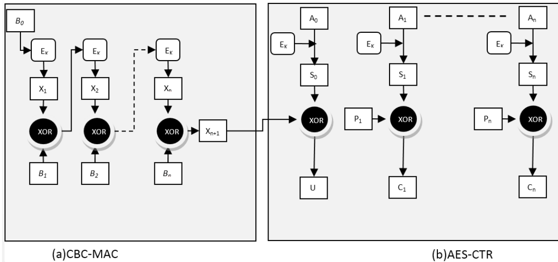
Figure5: Message encryption and authentication by AES-CCM
