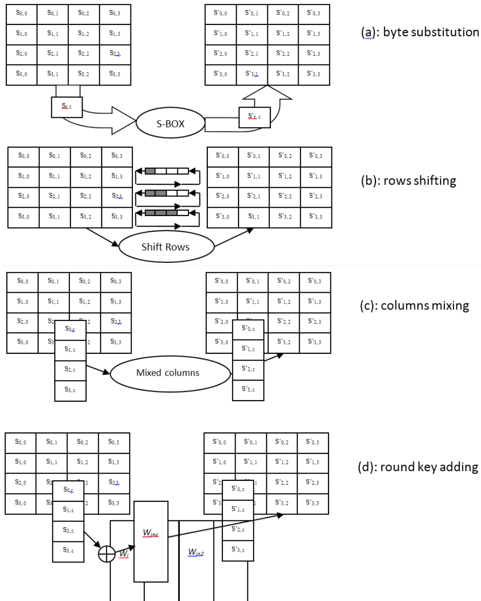
Figure 2: AES Cipher transformation
