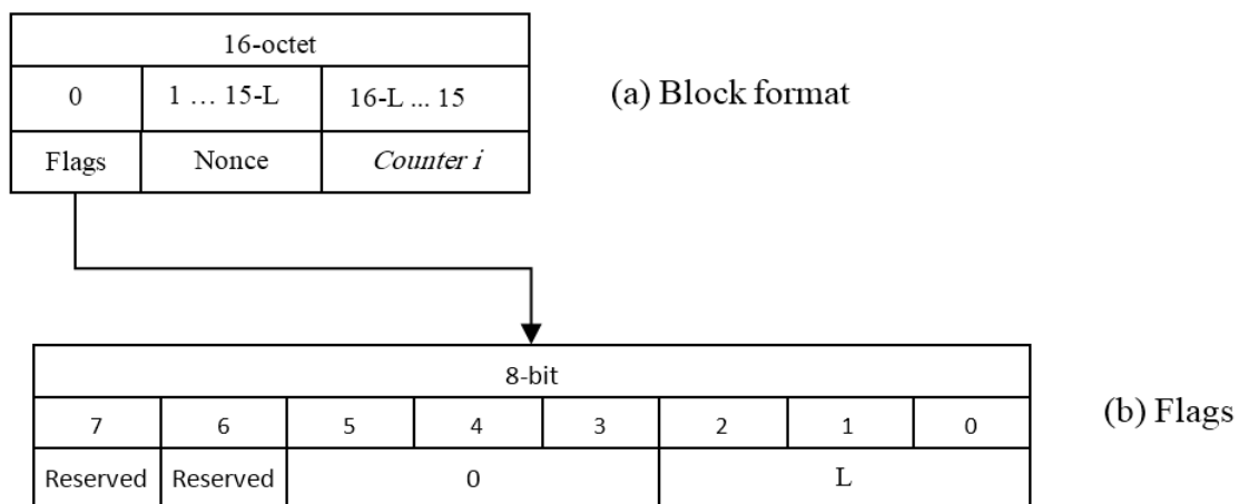
Figure 4: Block ( A_i ) and flags format
