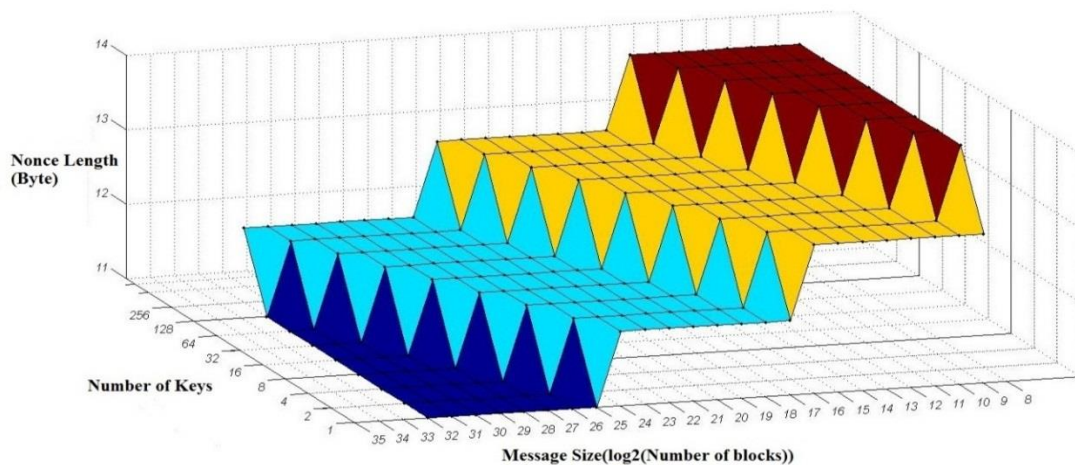
Figure9: Nonce length incremental over different number of secret key
