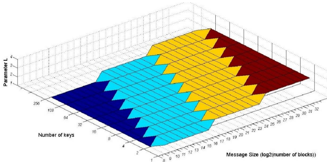
Figure8:Impact number of Secret keys on Parameter (L)
