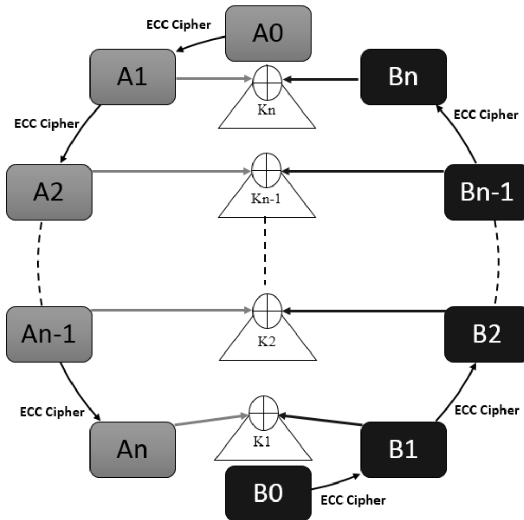
Figure 6: Multiple Secret Key Generation Protocol
