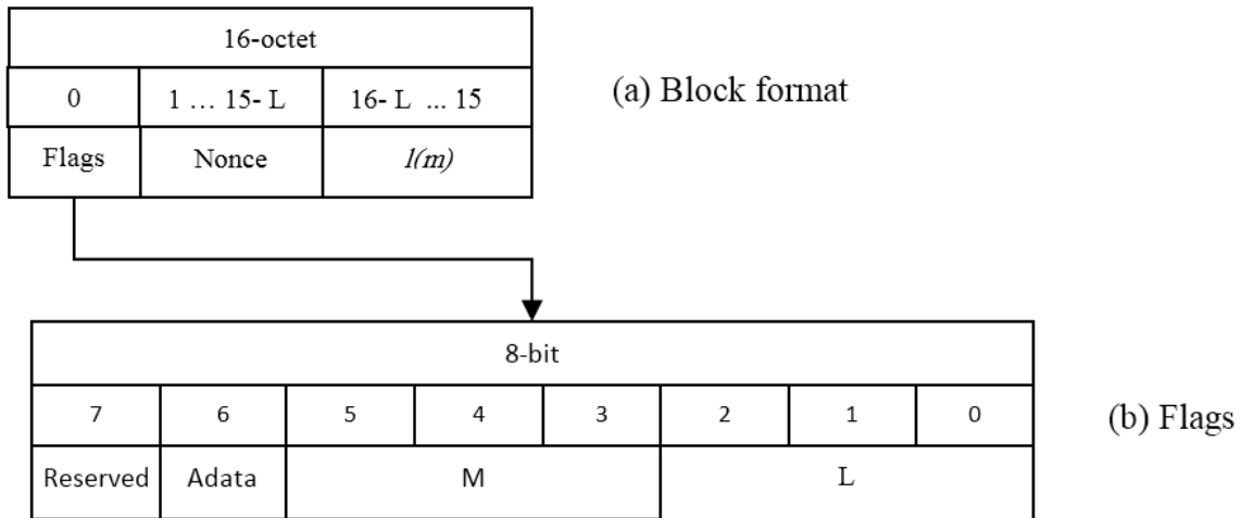
Figure3: Block ( B_0 ) and flags format
