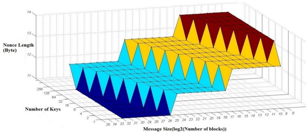
Figure9:shows the messages with size from 2^9 to 2^{16} had maximized their nonce length with number of secret keys ( 2^i ( i=1 to 8)) respectively.
