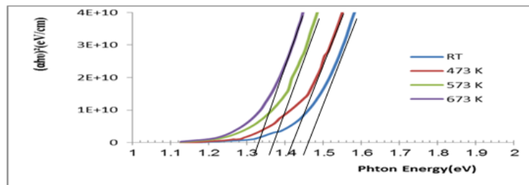
Figure (5): (\alpha h\nu)^2 change with photon energy ( h\nu ) of AIT thin films
