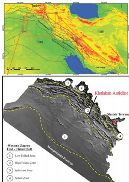
Fig. 2: Tectonic location of Khalakan Anticline [1]
