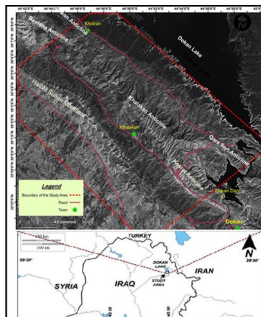
Fig. 1: Geomorphologic location of the studied area
