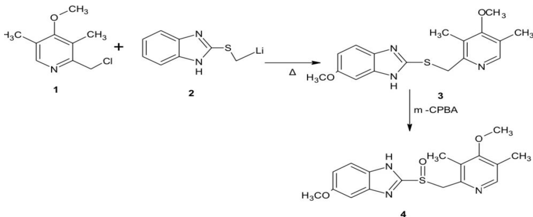
Fig. 5 The chemical reaction for preparing Omeprazole [64].
