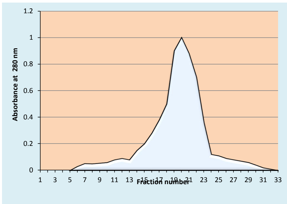
Figure 2 : Ion exchange chromatography of B.subtilis S4 by using ion exchange column (2.5 ×10 cm) ,with phosphate buffer , flow rate 100 ml/hr and 8 ml /fraction.
