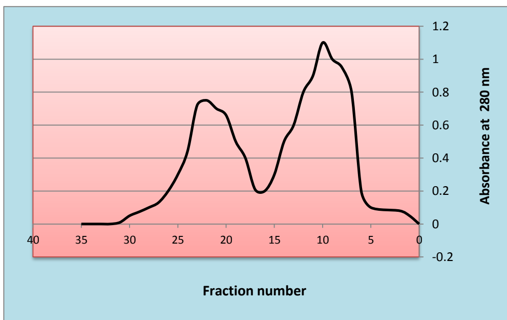
Figure 3: Gel filtration chromatography of B.subtilis S4 biosurfactant by using Sepharose-6B column (2.5 ×15 cm) with phosphate buffer , flow rate 100 ml / hr and 9 ml / fraction.
