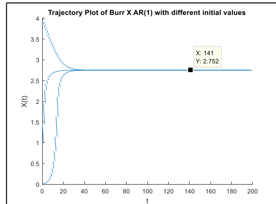
Fig (3.1): Trajectory plot of Model (3.15)
