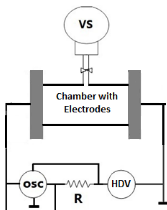
Figure 1. Experimental set-up
