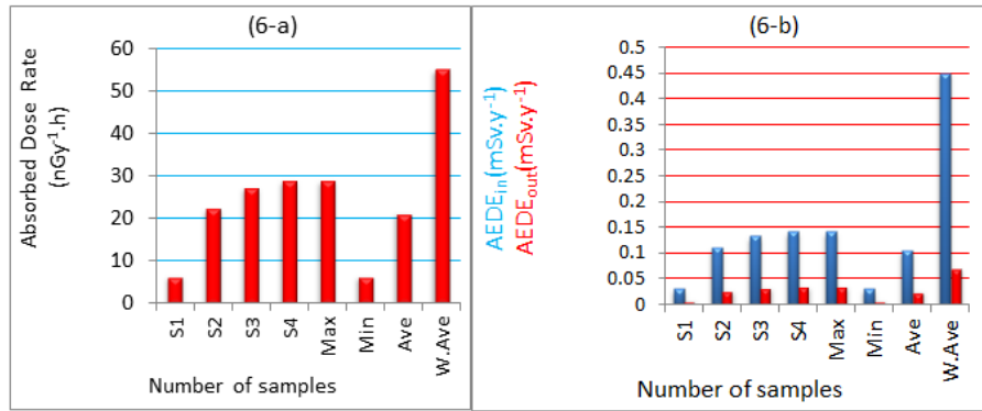
Fig (6-a): Show that the values of absorbed dose in air nGy.kg -1 in the soil sample.
