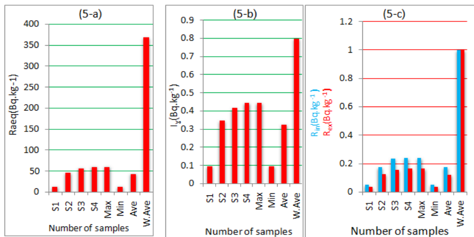
Figure (5-a): Show that the radium equivalent activity R_{eq} (Bq.kg -1 ) in the soil samples.
