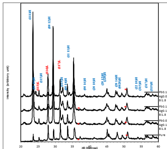
Figure (3) X-ray diffraction for compound \text{Bi}_{2-(x+y)}\text{Pb}_x\text{Ag}_y\text{Sr}_2\text{Ca}_2\text{Cu}_3\text{O}_{10+\delta} . After repeating the annealing.
