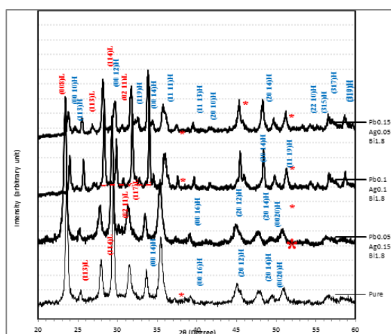
Figure (2) X-ray diffraction for compound \text{Bi}_2 .
