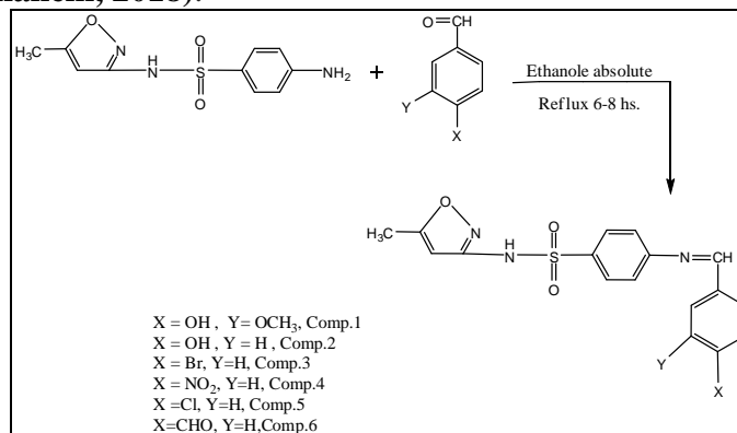
Scheme (1): The synthesis of Schiff's bases compounds from Sulfamethoxazole drug.
