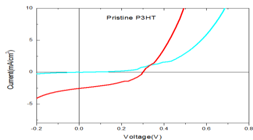
Figure 5: Current density vs. voltage measured on P3HT/ZnO nanowire arrays solid state dye for Pristine.
