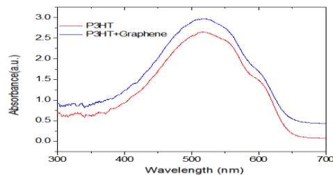
Figure 2: The optical absorption spectrum of the poly (3HT 5% wt) in the UV-visible-NIR range.
