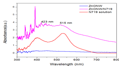
Figure 3: The Optical Absorption spectrum of ZnO NW, ZnO NW/N719, and N719 solution.
