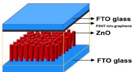
Figure 7: Schematic diagrams of the new-structure ZnO nanorod DSSC fabricate.
