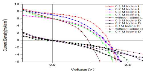
Figure 6: Current density vs. voltage measured on G-P3HT/ZnO nanowire arrays solid state dye with different loading of Iodine.
