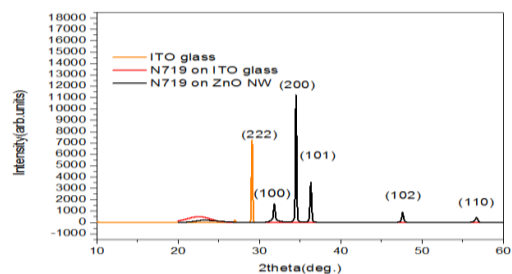
Figure 4: XRD spectrum of pristine N719 (red curve), N719 on ZnO NW arrays (black curve), and ITO (yellow).
