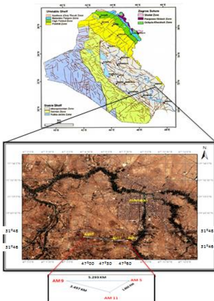
Figure 1: Tectonic subdivision of Iraq [8] and focusing in well studied area location with a Satellite image from (Sentinel-2 satellites) in Amara oil field
