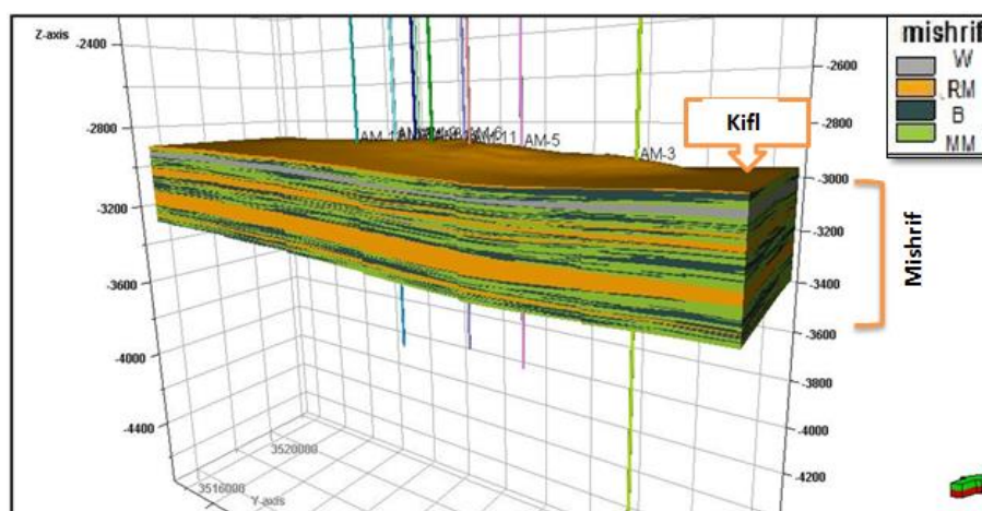
Figure (21) 3D Facies models of Mishrif and Kifl formations When the W:BP3,MM2,SCB4,CB3,RP1,RW2, Submicrofacies sequence . RM: RW1,RM3,RG1 submicrofacies B: SRB1,CB3,SCB1 submicrofacies and MM:MP2,MM2 submicrofacies .
