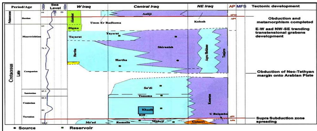
Figure 2: Stratigraphic correlation of studied formations in Late Early Turonian-Danian Megasequence[2]
