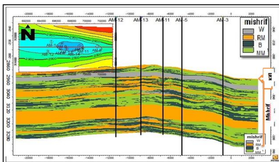
Figure(20)2D Facies models of Mishrif and Kifl formations the W:BP3,MM2,SCB4,CB3,RP1,RW2, Submicrofacies sequence . RM: RW1, RM3,RG1 submicrofacies B: SRB1,CB3,SCB1 submicrofacies and MM:MP2,MM2 submicrofacies .
