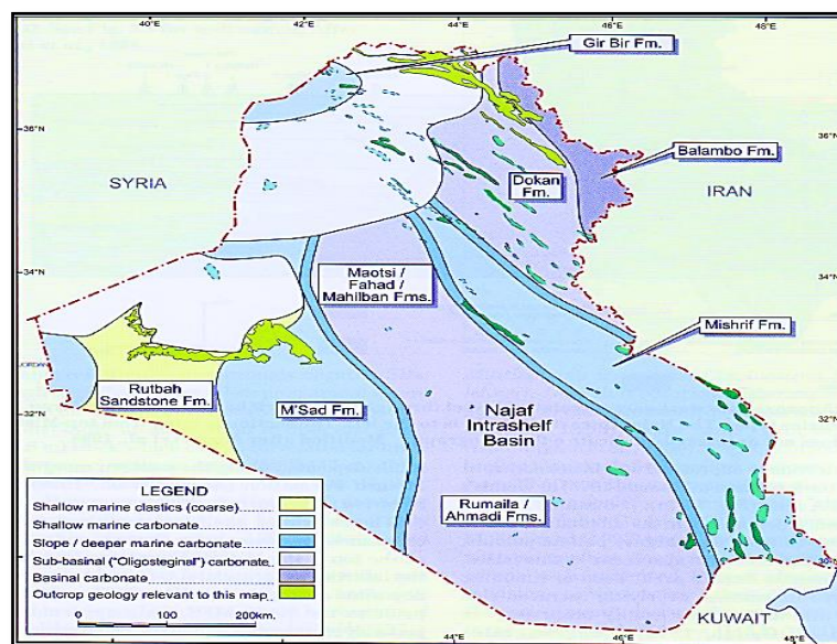
Figure 3: Paleogeography of Latest Albian-Early Turonian in Iraq from [2]
