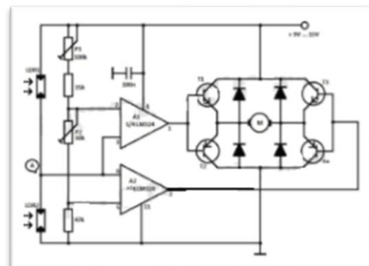
Figure (3) see electronic circuit of tracking
