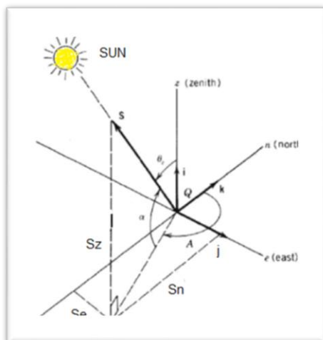
Figure (1) Earth surface coordinate system for observer at Q
