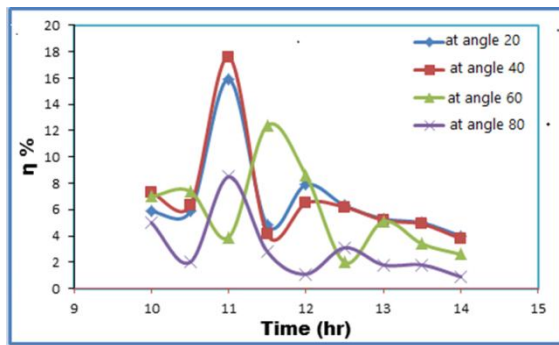
Figure (8) illustrates the relationship between efficiency and time at different angles
