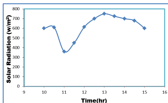
Figure (7) solar radiation with time at cloudily day
