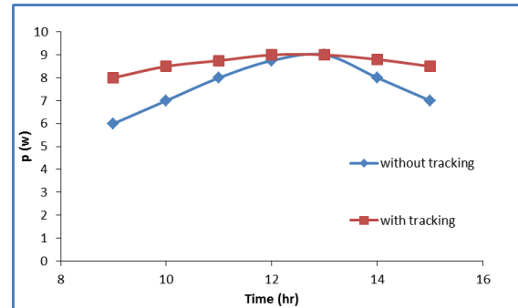
Figure (9) Show the relation of power with and without tracking with time
