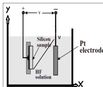
Figure (2) A schematic diagram of the electrochemical cell.
