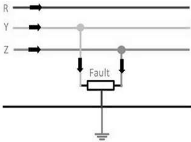
Figure 3: Double line to ground fault
